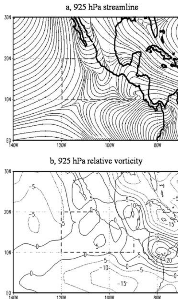
Fig. 14. Same as Fig. 13, except for 1977.
