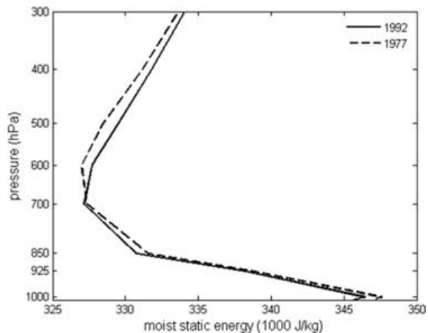
Fig. 3. Vertical profile of seasonal mean moist static energy averaged over 90°–120°W and 10°–20°N in 1992 (solid) and 1977 (dashed).
