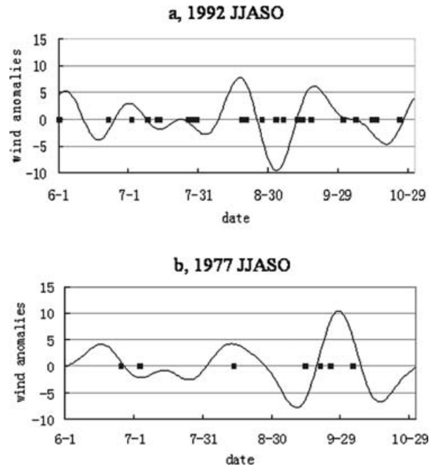
Fig. 11. Time series of 30–50-d filtered 850 hPa zonal wind anomalies ( \text{m s}^{-1} ) during June to October in (a) 1992 and (b) 1977 over the locations denoted by the solid dots in Fig. 10. Solid squares denote the timing of cyclogenesis.
