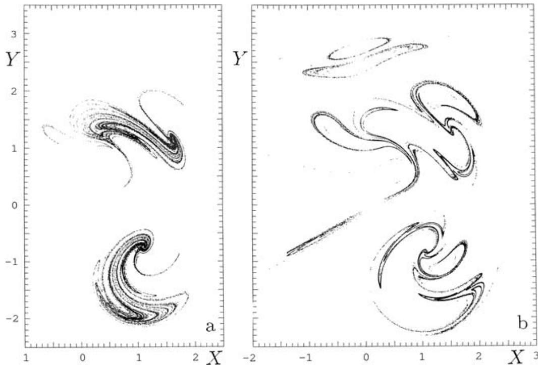
Fig. 3. (a) Intersection with plane Z = 0 of attractor of approximation to eqs. (1), when a = 1/4 , b = 4 , F = 8 and G = 1 , by first-order differencing with \tau = 0.037 . Coordinates are X and Y . (b) The same, but with \tau = 0.042 .
