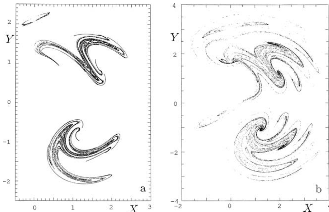
Fig. 1. (a) Intersection with plane Z = 0 of attractor of eqs. (1) when a = 1/4 , b = 4 , F = 8 and G = 1 , as represented by 97 428 points computed with fourth-order Taylor-series procedure with time increment \tau = 0.025 . Coordinates are X and Y . (b) The same, but with 168 266 points, and when a = 1/4 , b = 5 , F = 14 and G = 7/4 . Note the change in scale.
