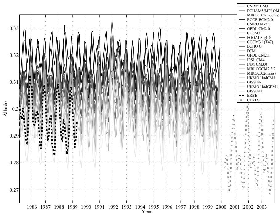
Fig. 1. Global monthly mean albedo time series from 20 GCMs (solid grey lines) compared with ERBE and CERES satellite observations (dashed black lines).
