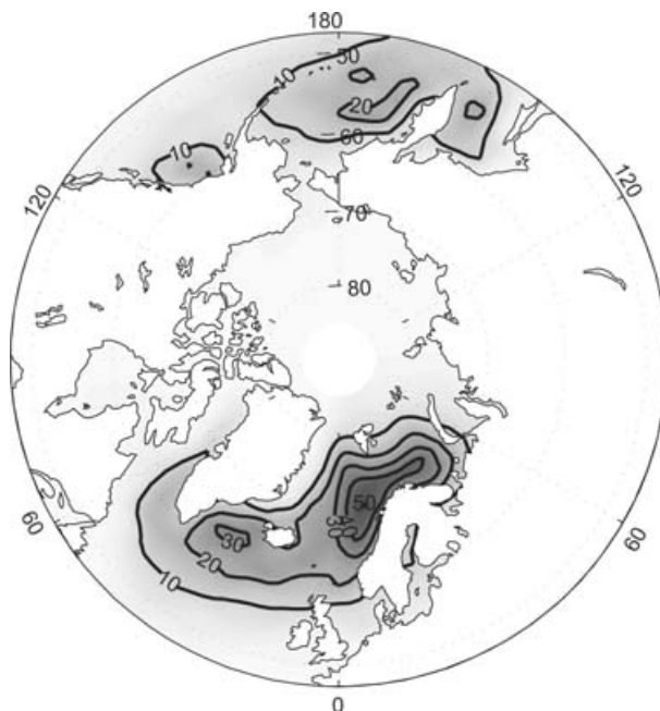
Fig. 15. As in Fig. 13, but now with the low stability constraint only.
