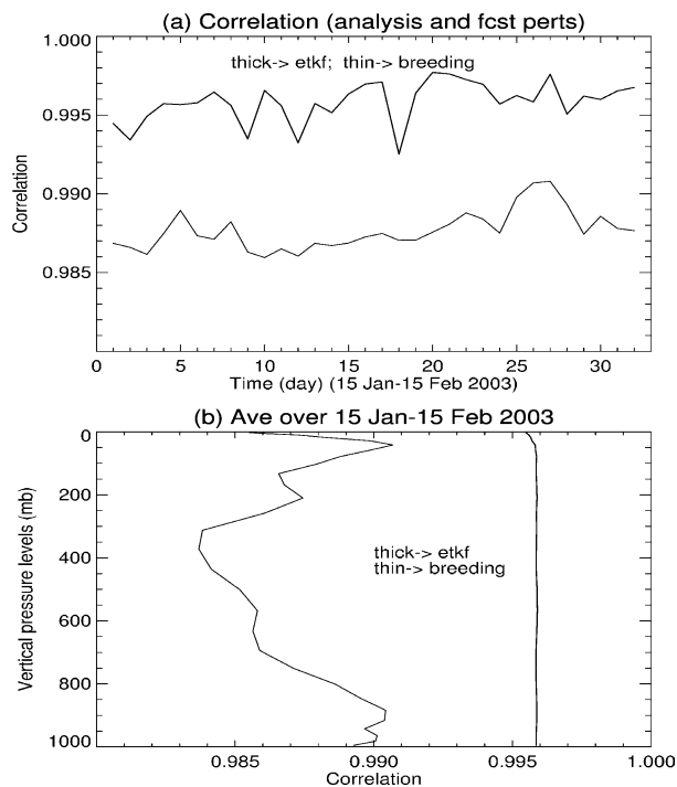
Fig. 11. Averaged correlation over 10 members between forecast and analysis perturbations for ETKF (thick) and breeding (thin) ensembles; (a) mean correlation as a function of time over all levels and (b) vertical correlation distribution averaged over time.
