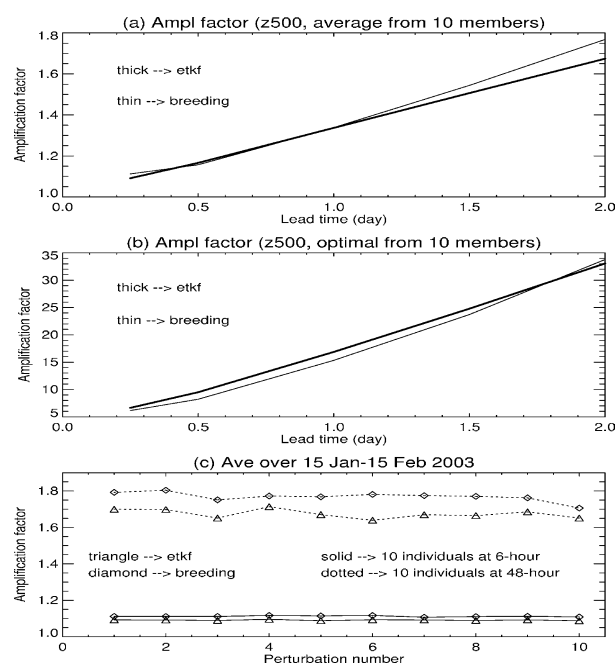
Fig. 8. Amplification factors of ensemble perturbations for (a) the average AF from 10 perturbations as a function of lead time (thick: ETKF; thin: breeding); (b) the maximum AF of optimally combined orthogonal perturbations from 10 original perturbations (thick: ETKF; thin: breeding); (c) the AF of 10 individual perturbations for two forecast lead times (solid: 6-hr; dotted: 48-hr; triangle: ETKF; diamond: breeding).
