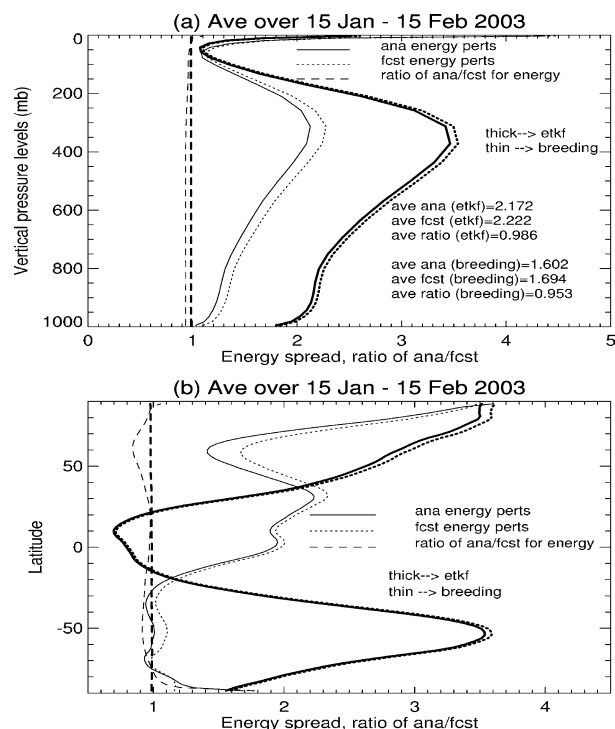
Fig. 3. Energy spread distributions of ETKF (thick) and breeding (thin) ensemble perturbations (solid: analysis; dotted: forecast). The ratio of analysis/forecast perturbations is indicated by the dashed line. All the values are averaged over the period 15 January–15 February 2003, with (a) vertical distribution as a function of pressure; (b) distribution by latitude.
