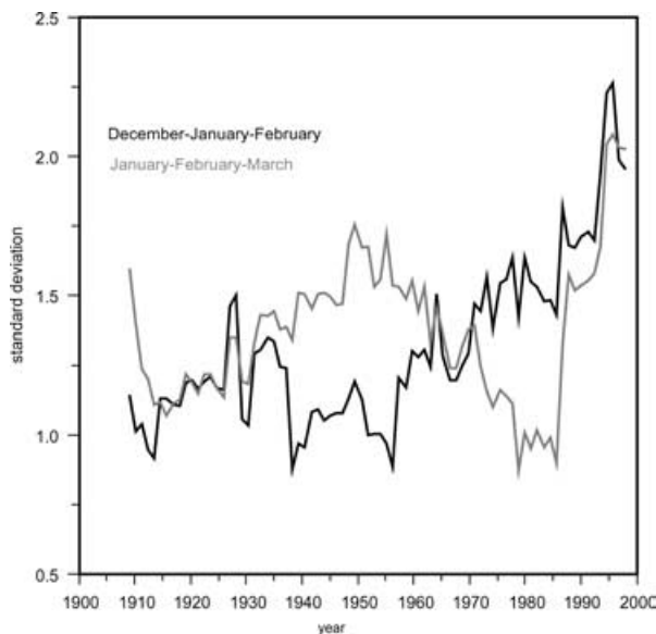
Fig. 4. Comparison between the moving standard deviations (21-year window) of two different winter NAO indices, December–February and January–March.
