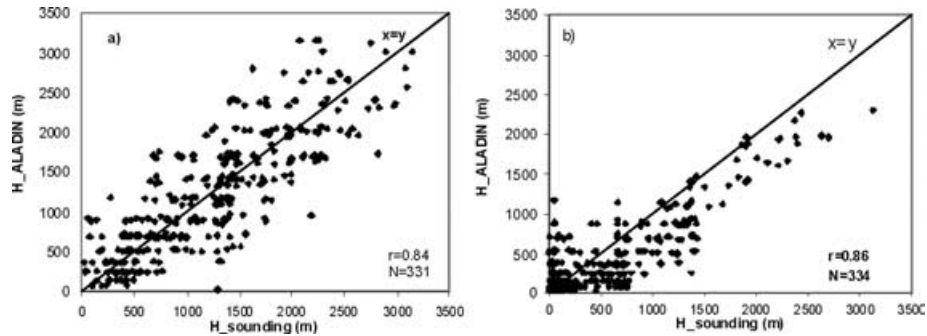
Fig. 2. Scatter plots comparing H calculated at (a) 12 UTC for (Ri_{Bc\_soundings}, Ri_{Bc\_ALADIN})_{day} = (0.2, 0.4) and (b) 00 UTC for (Ri_{Bc\_soundings}, Ri_{Bc\_ALADIN})_{night} = (1.5, 1.5) for 10 April 2003–10 April 2004 in Zagreb, Croatia.
