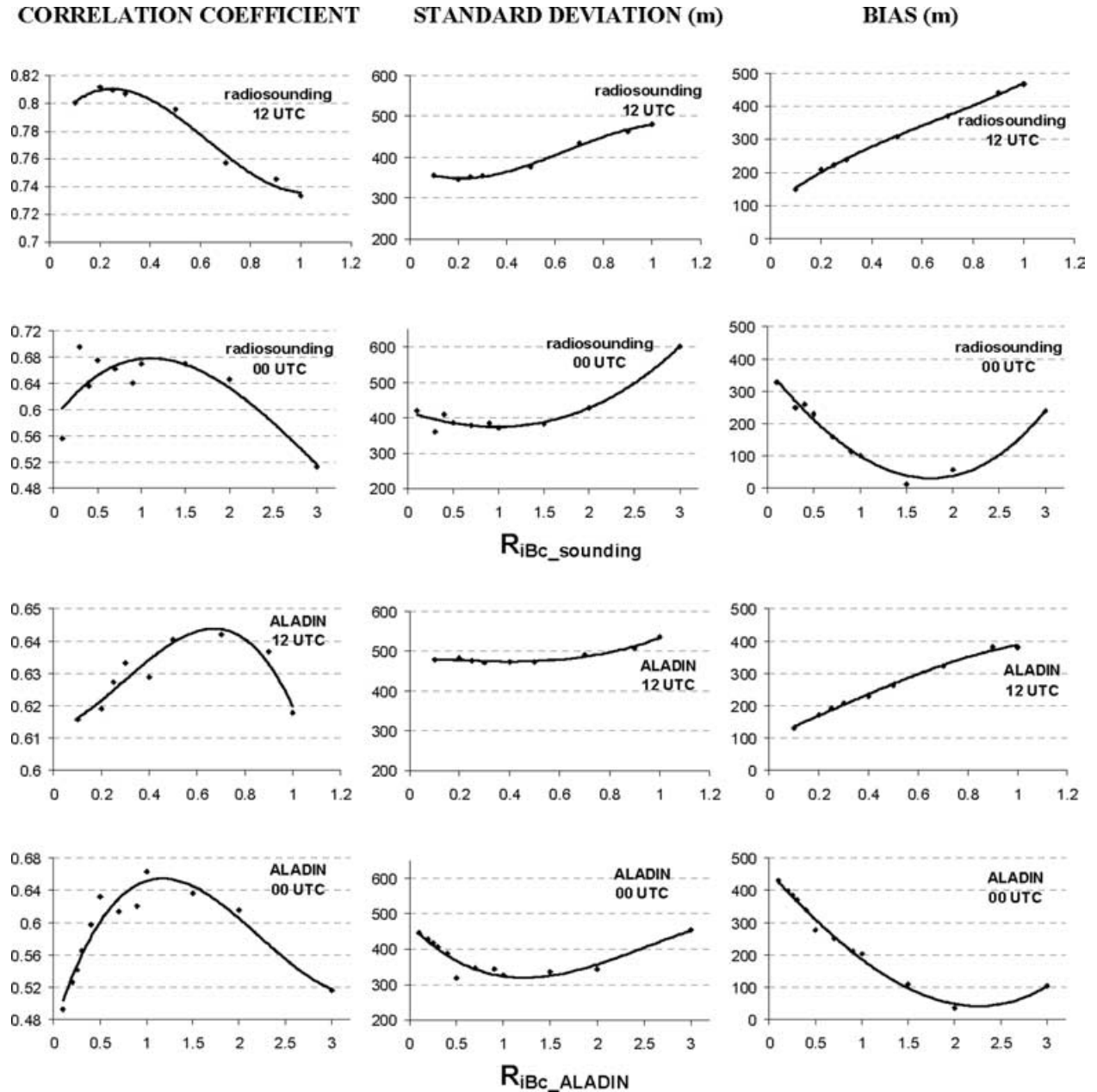
Fig 5. The correlation coefficient, standard deviation and absolute bias between: H_{\text{soundings}} , H_{\text{ALADIN}} and H_{\text{Holzworth}} at 12 UTC and 00 UTC for different Ri_{Bc} for period 10 April 2003–10 April 2004 in Zagreb, Croatia. Subfigures are self-explanatory and similar to the earlier plots.
