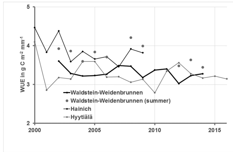
Fig. 5. Water use efficiency of three sites calculated as the ratio of annual sums of GPP and ET. Because of this simplification, for Waldstein-Weidenbrunnen site measurements in summer were calculated from the available single measured data (not gap-filled).
