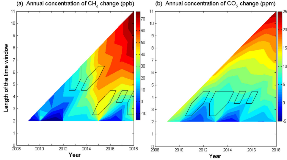
Fig. 7. Change of (a) CH 4 (ppb) and (b) CO 2 (ppm) concentrations recorded at the LTO station from May 2008 to August 2018 as a function of length of time window ( y -axis) and ending of year of calculation. The inside of the black contours shows significant areas with a 95% confidence level from the student's t -test.
