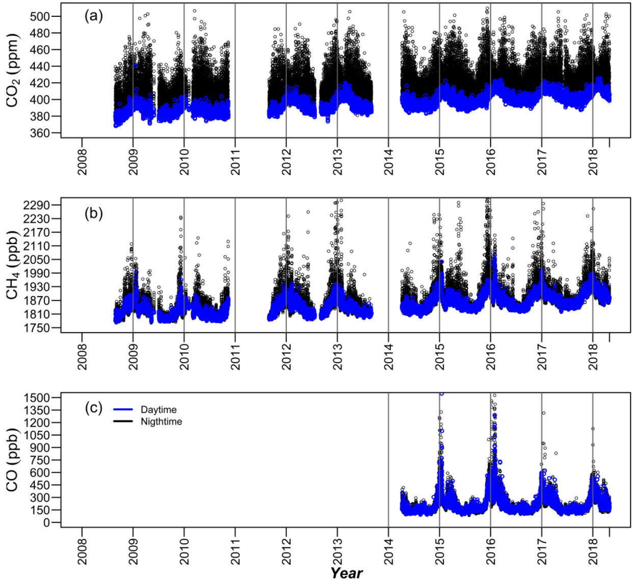
Fig. 5. Time series of atmospheric CO 2 (a), CH 4 (b) and CO (c) concentrations measured at the LTO station over the 2008-2018 period. The blue colour represents day-time data (from 11 h to 17 h) and the black colour represents night-time data (from 17 h to 11 h). The vertical lines differentiate years.
