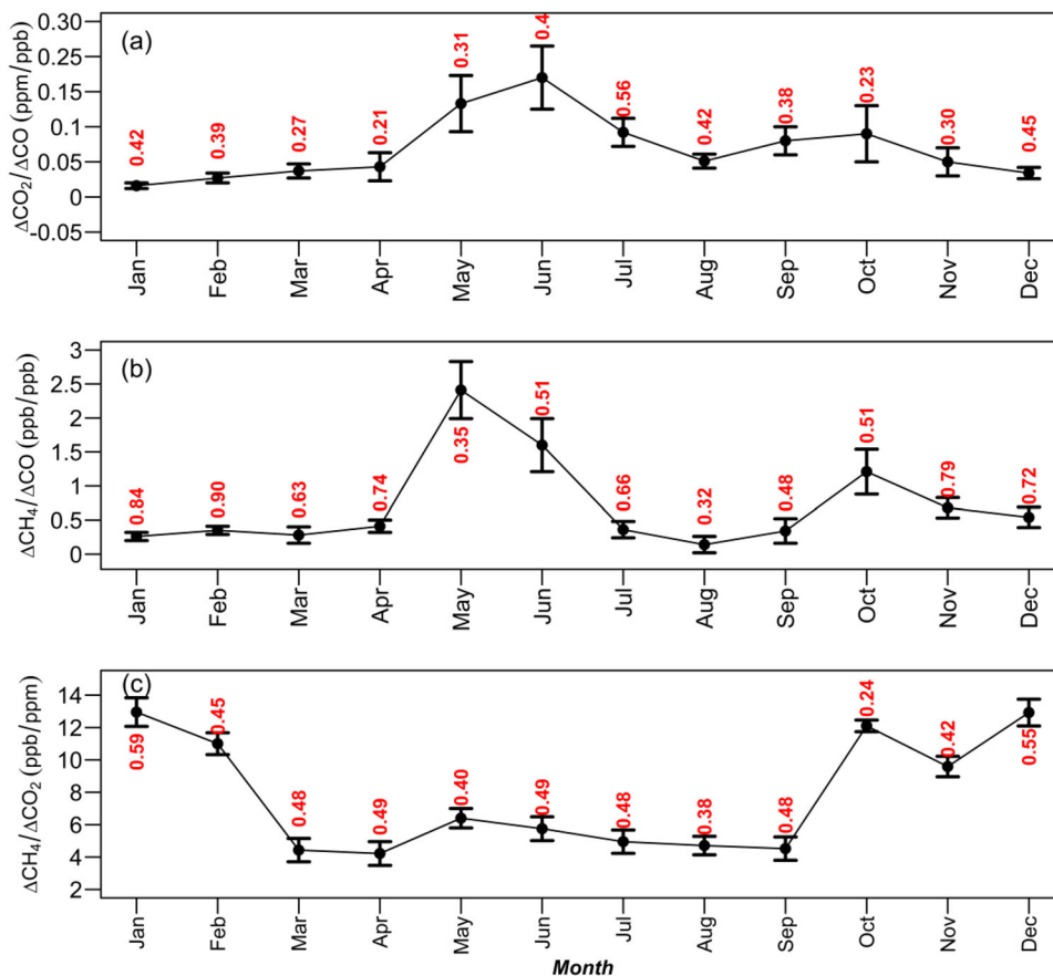
Fig. 10. Mean monthly variations (in black lines) of (a) \Delta\text{CO}_2/\Delta\text{CO} , (b) \Delta\text{CH}_4/\Delta\text{CO} and (c) \Delta\text{CH}_4/\Delta\text{CO}_2 obtained from the dispersion pattern slopes between the \text{CO}_2 , \text{CH}_4 and \text{CO} residues at the LTO station over the 2014-2018 period. The numbers in red are the correlation coefficients between each pair of species. Vertical black bars represent standard deviation.
