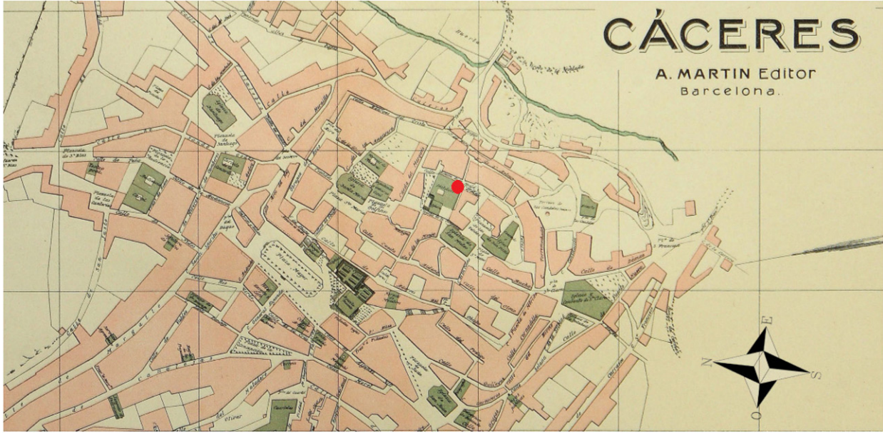
Fig. 2. Old map of the city of Cáceres (Spain) showing the position of the meteorological station located at the terrace of the High School.
