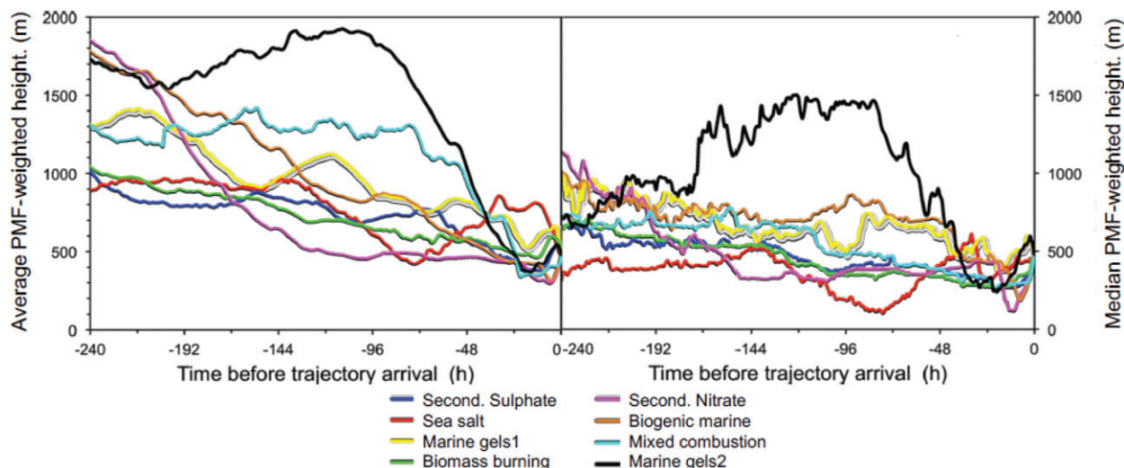
Fig. 6. Left: Average PMF-weighted trajectory heights during 240 h before air mass arrival at the receptor site at 474 m a.s.l., related to the maps in Fig. 5; right: PMF-weighted 50 percentiles trajectory heights.
