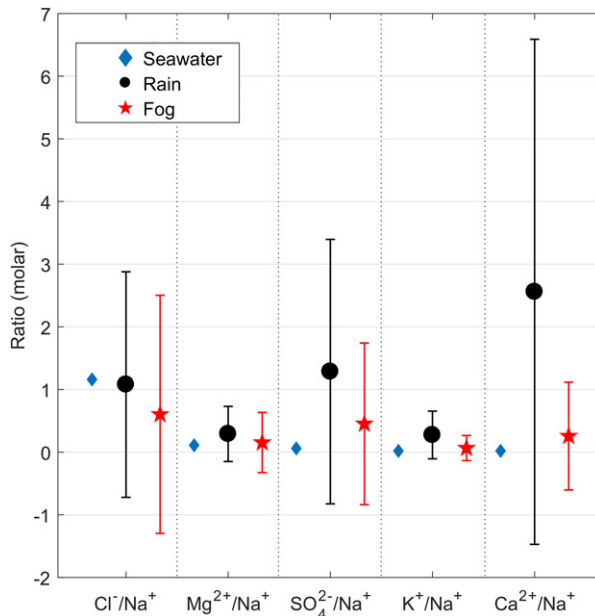
Fig. 3. Sea-salt ratios referred to \text{Na}^+ in bulk seawater (blue diamonds), in rain (black circles) samples, and in fog (red stars) samples collected during the CAEsAR campaign. Fog/rain ratios were calculated using mean ion concentrations. Error bars represent 1\sigma .
