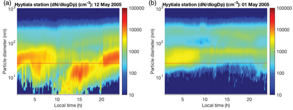
Fig. 1. Examples of an event (a) and a non-event (b) day at Hyytiälä, Finland, in May 2005. The x -axis shows one 24-h time period whereas the y -axis shows the range of particle size diameters (from 3 to 1000 nm). The color scale indicates particle concentration ( \text{cm}^{-3} ). In (a) one can clearly see aerosol particles forming around noon and then growing into larger sizes. This data was accessed via Smart-SMEAR (Junninen et al., 2009).
