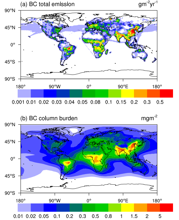
Fig. 1. Spatial distribution of (a) BC emissions ( \text{g m}^{-2} \text{ yr}^{-1} ) in 2005 and multi-year (50-year) mean (b) BC column burden ( \text{mg m}^{-2} ).
