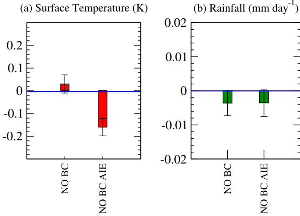
Fig. 5. Global mean annual average changes in (a) surface temperature (K), and (b) rainfall ( \text{mm day}^{-1} ) from the coupled model simulations. Error bars indicate the 95% confidence interval on the error in the mean.
