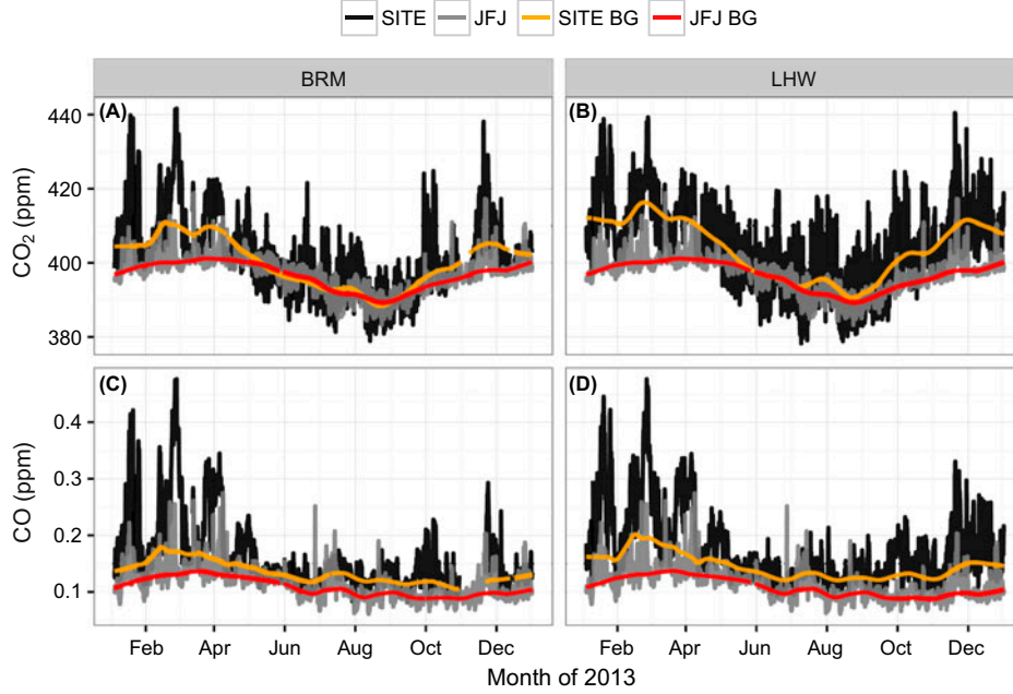
Fig. 4. CO 2 (panels A–B) & CO (panels C–D) measured mole fractions (black and gray) and ‘robust estimate of baseline signal’ (REBS) estimates (red and orange) at Beromünster, Lägern-Hochwacht, and Jungfrauoch (JFJ) during 2013. The REBS background estimates are calculated with a 45-day local regression window.
