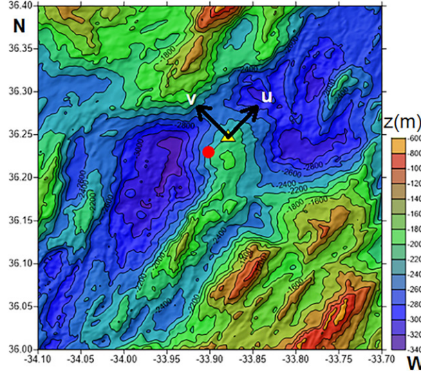
Fig. 2. Bathymetric map part of the Mid-Atlantic Ridge, southwest of the Azores (P). The site of the mooring is indicated by the yellow triangle centring the positive directions of the local along- and cross-slope current components on the north-slope of Rainbow crest. The red dot indicates Rainbow's main hydrothermal vent. Multibeam data, 100 \times 100 m grid.
