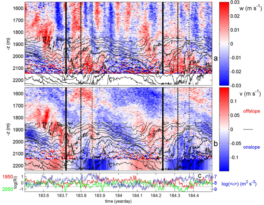
Fig. 3. One day of data around Fig. 1 of high-resolution 398-m range T-observations superposed on low-resolution 600-m range ADCP observations. (a) Vertical current component, smoothed over 600s intervals. Black contours indicate \Theta every 0.05^\circ\text{C} . The seafloor is at the horizontal axis. The black-solid vertical bars indicate approximate times of internal turbulence expansion, the thick dashed lines those of pre-frontal mixing (van Haren et al., 2017) and the dash-dotted lines those of near-bottom frontal bore. Each set of lines is shifted an exact multiple of the semidiurnal lunar tidal period. (b) Cross-slope current component with the lower 95-m thick bar coloured by the current meter data at 7 mab (up to the lowest bin of good ADCP-data at 100 mab). Black contours are copied from a. for reference. (c) Logarithm of gradient Richardson number for hourly smoothed 100-m-averaged values around z = -1950 m (red) and z = -2050 m (green), with horizontal black lines indicating (in)stability transition values of 0.25 (solid; Miles and Howard, 1964) and 1.0 (dashed; Abarbanel et al., 1984). Additionally, the logarithm is given of the record of vertically 8–405 mab-mean dissipation rate (in blue, scale to right).
