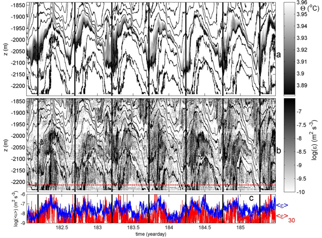
Fig. 5. Three-and-a-half days of data around Fig. 1 demonstrating the straining and off-bottom turbulent bursting varying every tidal period. (a) Conservative temperature. Black contours are drawn every 0.09^\circ\text{C} . The seafloor is at the horizontal axis. The black-solid vertical lines indicate approximate times of internal turbulence expansion. The lines are shifted by an exact multiple of the semidiurnal lunar tidal period. (b) Logarithm of un-averaged dissipation rate from data in a. using the method of Thorpe (1977), with black contours copied from a. for reference. The red horizontal dashed line is at 30 mab. (c) Logarithm of vertically averaged dissipation rate, in blue for the entire temperature sensor range between 8 and 405 mab, in red for near-bottom 8 to 30 mab.
