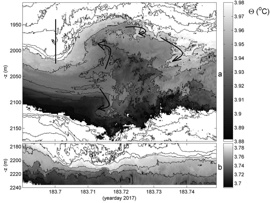
Fig. 1. Example of detailed off-bottom >100-m tall turbulence expansion burst from 1.5 h of high-resolution conservative ( \sim potential) temperature data observed on July 2 (year day 183) between 8 and 405 m above the bottom ‘mab’, with 19 flawed T-sensors interpolated. Black contours are drawn every 0.02 °C. (a) Middle 268 m of the T-sensor range. The black vertical bar indicates the transition moment to supercritical flow, the arrows some overturning interpretations. (b) Lower 65 m above the bottom (seafloor = horizontal axis) with different colour ranges.
