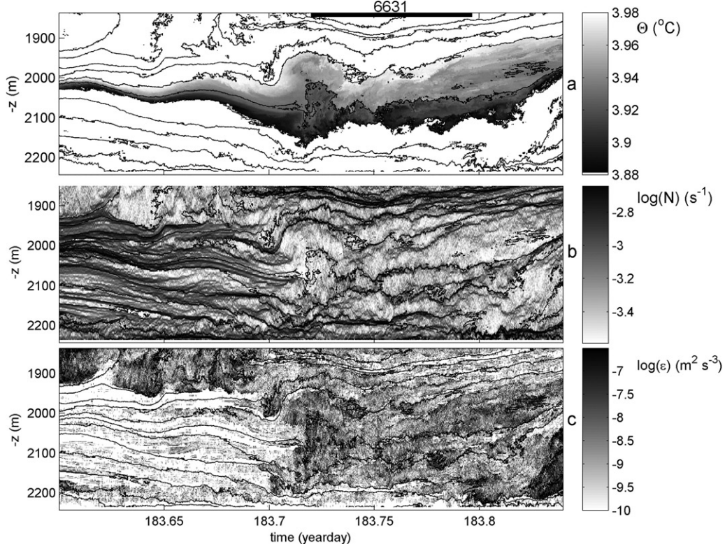
Fig. 4. Six hours of data around Fig. 1 from high-resolution T-sensor data. (a) Conservative Temperature. Black contours are drawn every 0.05^\circ\text{C} . The horizontal bar indicates the mean buoyancy period (in s) for the entire panel. The seafloor is at the horizontal axis. (b) Logarithm of buoyancy frequency from reordered \Theta , with black contours copied from a. for reference. (c) Logarithm of un-averaged dissipation rate from data in a. using the method of Thorpe (1977), with black contours copied from a. for reference.
