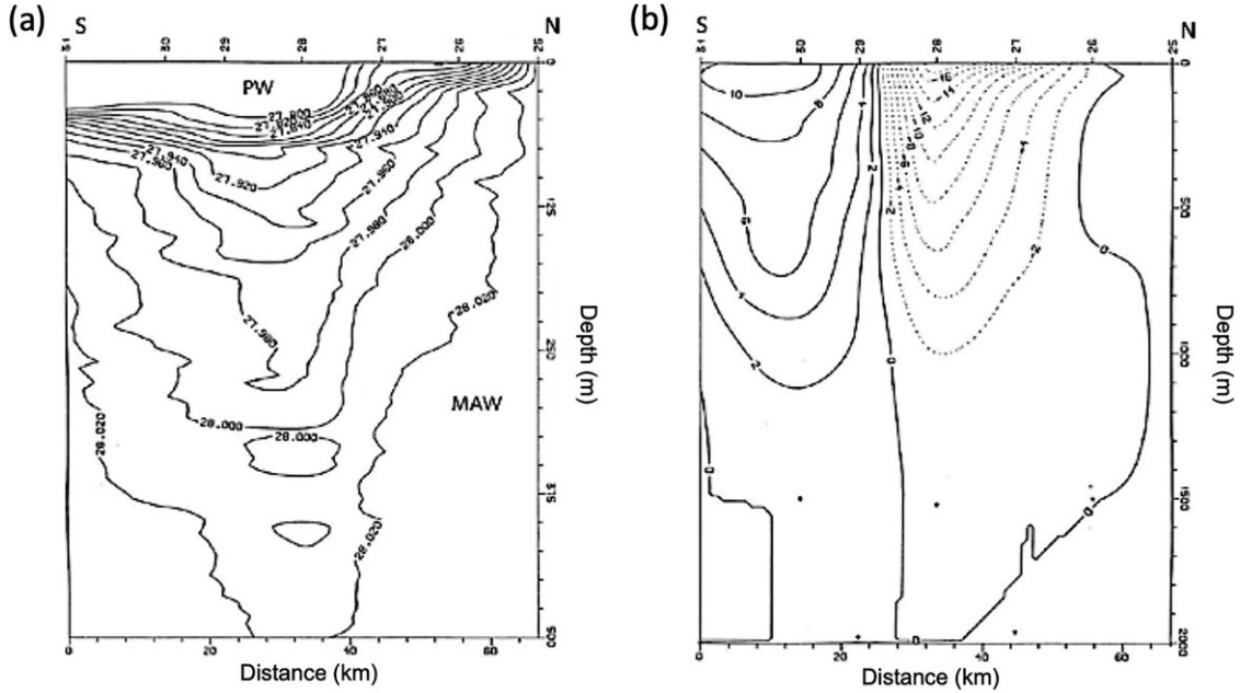
Fig. 4. The anticyclonic eddy characteristics. a, Density section of the North (N)–South (S) section on 2 April shown in Fig. 3e. b, Geostrophic current in the N–S section with 0 reference level at 2000 m. Dotted lines: eastward current; full lines: westward current in cm/s. Note the different y-axis scale for the depth, 500 m for a and 2000 m for b. The section is 65-km long and with station spacing of 8–11 km.
