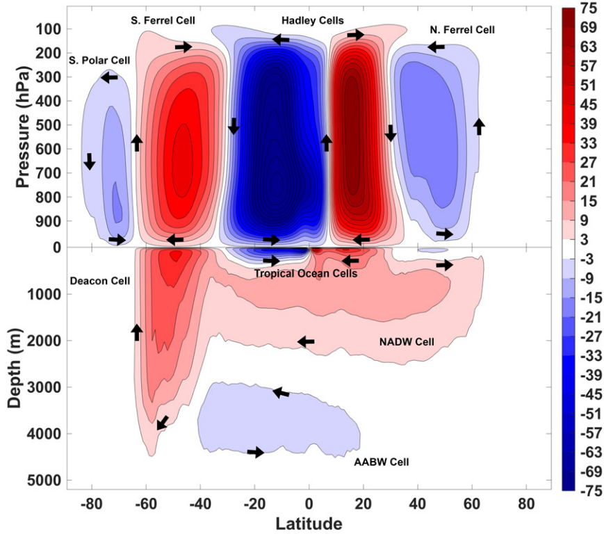
Fig. 1. The global air-mass overturning stream function for the atmosphere (top panel) and global water-mass overturning stream function for the ocean (bottom panel). Arrows indicate the mass transport direction. N represents the Northern Hemisphere and S is used for the Southern Hemisphere. NADW stands for North Atlantic Deep Water and AABW represents Antarctic Bottom Water. All transports are in Sv ( 10^9 kg/s).
