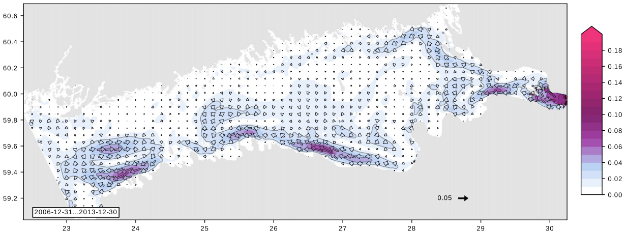
Fig. 2. Annual mean circulation averaged from 0 to 7.5m depth for the years 2007–2013. Velocities are in m/s. Vector arrows are drawn for every 15 grid points in the longitudinal direction and every 13 grid points in the latitudinal direction.
