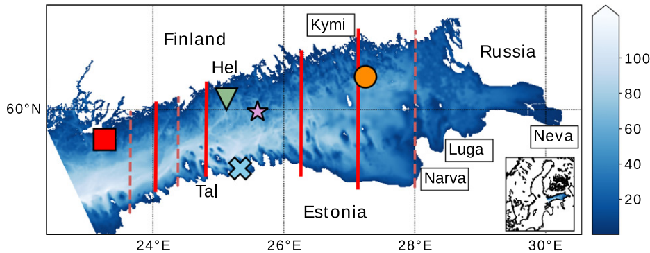
Fig. 1. The model domain and bathymetry (in metres). CTD stations referenced in the article (from the east): Haapasaari (orange circle), Länsi-Tonttu (green triangle) and Längden (red square). Kalbådagrund weather station is marked with a magenta star. Station 18A used in analysis is marked with a blue X. Red lines show the location of the transects used in the analysis. Solid, darker lines indicate transects that were used for plots in this article. The map also indicates the approximate location of the Neva river mouth at the eastern end of the basin, along with Kymi, Luga and Narva rivers. Furthermore, approximate locations of the cities of Helsinki (Hel) and Tallinn (Tal) are shown. The inset is the location of the model domain on a map of the Baltic Sea.
