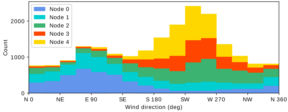
Fig. 12. Wind direction distribution for BMU's of SOM nodes as a stacked histogram, 2007–2013. Wind direction taken from the model forcing at the Kalbådgrund station. BMU from the section at 24.04°E.
