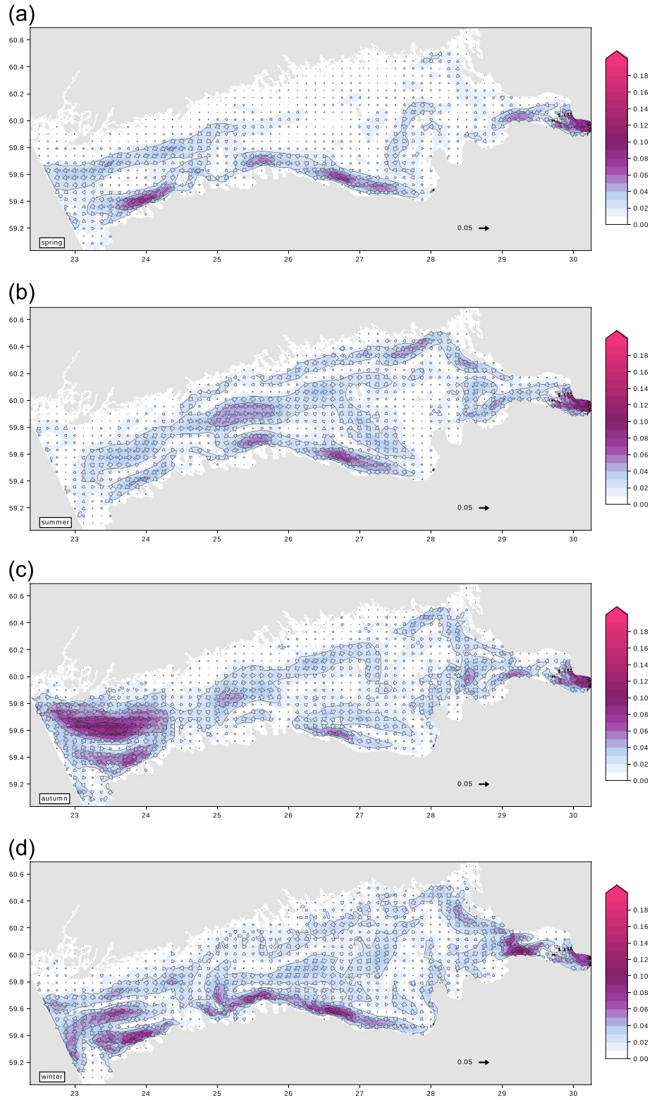
Fig. 3. Mean circulation in 2007–2013 averaged from 0 to 7.5m depth for spring (top), summer, autumn and winter (bottom). Velocities are in m/s. Vector arrows are drawn for every 15 grid points in the longitudinal direction and in every 13 grid points in the latitudinal direction.
