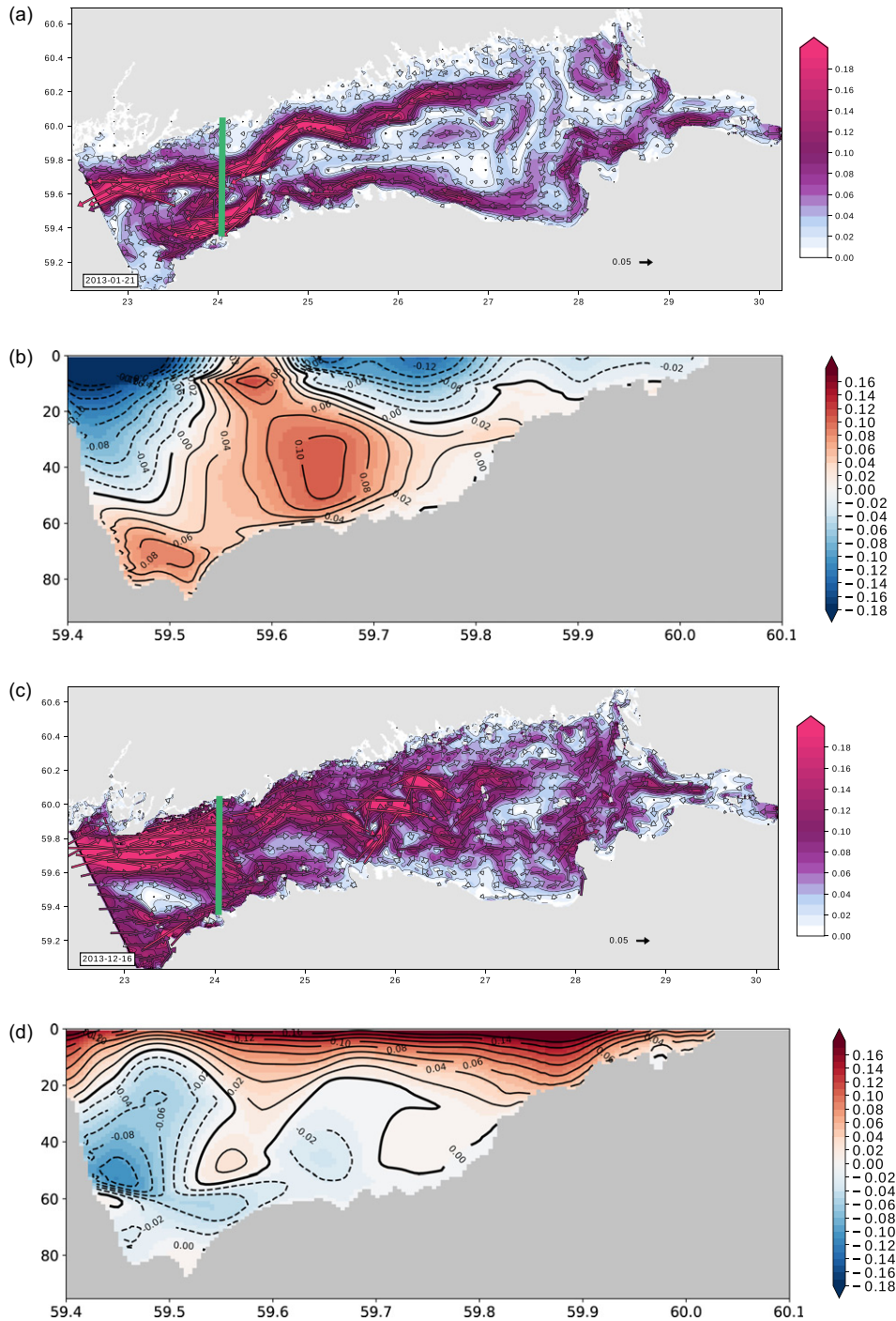
Fig. 9. Daily mean velocity maps and zonal component of velocity at north-south section at 24.04°E for 21 January 2013 (normal estuarine circulation) and 16 December 2013 (reversed estuarine circulation). Vector arrows are drawn for every 19 grid points in the longitudinal direction and every 17 grid points in the latitudinal direction. Location of the north-south section is indicated by a green line on the velocity maps.
