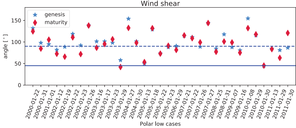
Fig. 5. Wind shear at genesis (blue stars) and maturity (red diamonds) stages. Blue lines separate forward (below blue thick line; 45^\circ ) and reverse (above blue dashed line; 90^\circ ) shear.
