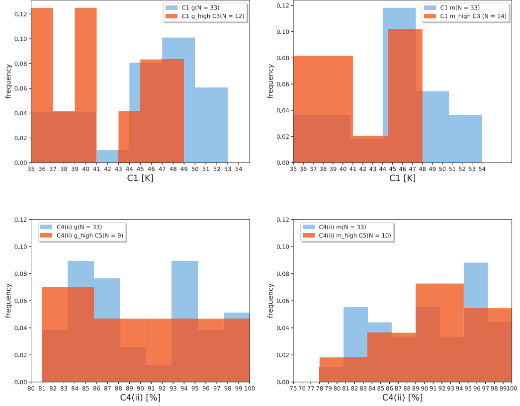
Fig. 4. Frequency of occurrence of condition C1 for all 33 cases (blue) and for cases with C3 above mean 75 percentile value of ASRv2 (orange) at genesis (g) (upper left) and maturity (m) (upper right) stages. Similar is shown for conditions C4(ii) with high C5 (above threshold) (bottom).
