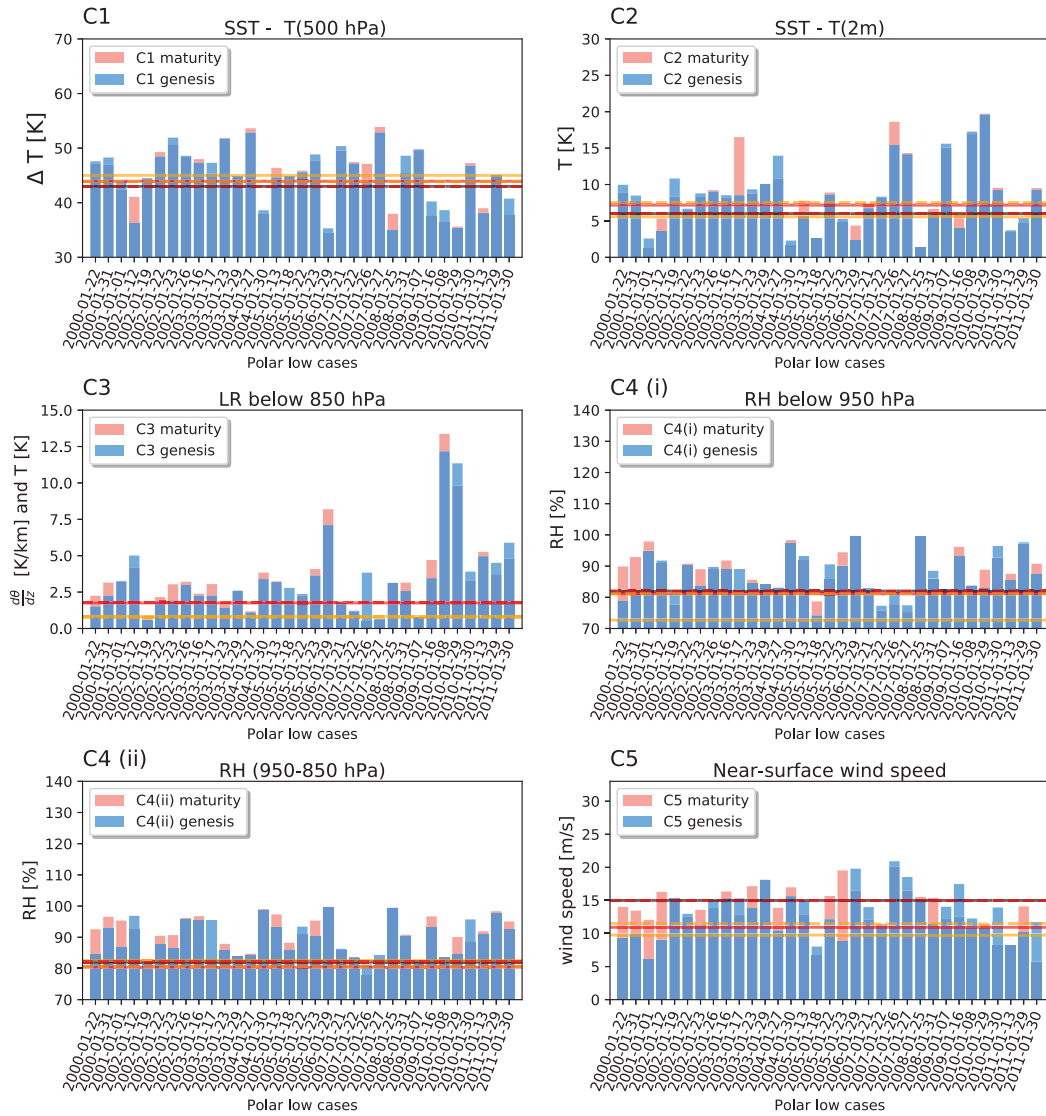
Fig. 3. Bars represent the values for the different conditions based on ASRv2 grid points within a 200 km radius around the genesis (blue) and maturity (orange) point for each of the January cases between 2000 and 2011. C1 (upper left), C2 (upper right), C3 (middle left), C4(i) (middle right), C4(ii) (bottom left) and C5 (bottom right). Horizontal lines represent: the literature threshold from Table 1 (black), ASRv2 mean (red) and ASRv1 mean (yellow) for genesis (maturity) stage denoted with full (dashed) line.
