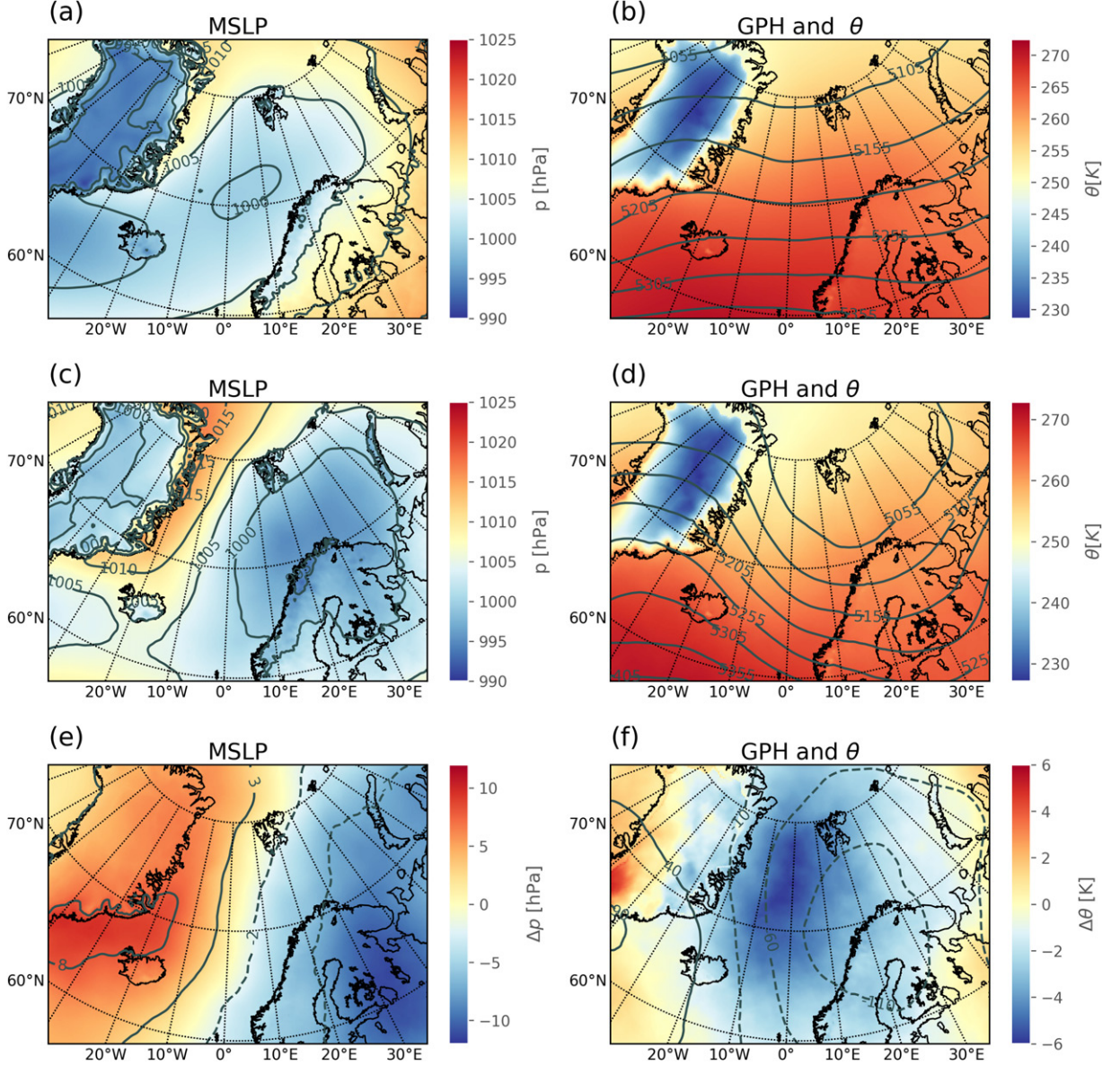
Fig. 9. Climatology of: (a) all 372 January days for MSLP (colour shading and grey-labeled counters, every 5 hPa) and (b) GPH at 500 hPa (grey-labeled contours, every 50 gpm) and potential temperature at 850 hPa (colour shading); (middle) As in the first row but for PL dates; (bottom) anomalies for both, MSLP (grey-labeled contours, every 5 hPa) (e) and GPH at the 500 hPa level (grey-labeled contours, every 50 gpm) and potential temperature (colour shading) (f).
