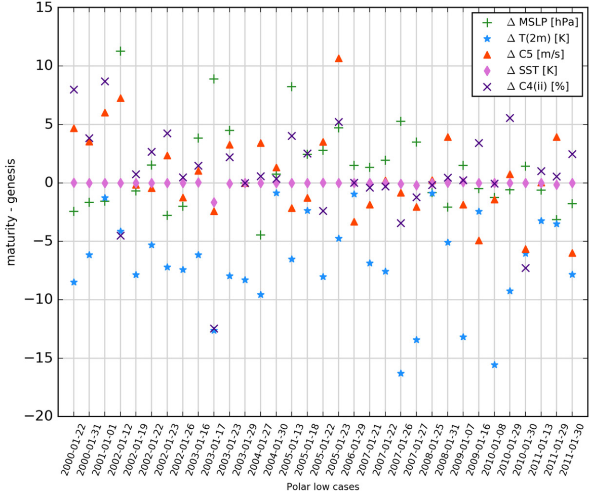
Fig. 7. Difference of environmental conditions between the genesis and the maturity stage. Shown are: MSLP difference (green pluses), temperature at 2 m (blue stars), near-surface wind speed (C5), SST, and RH in the layer between 850 and 950 hPa, C4(ii) (indigo crosses).
