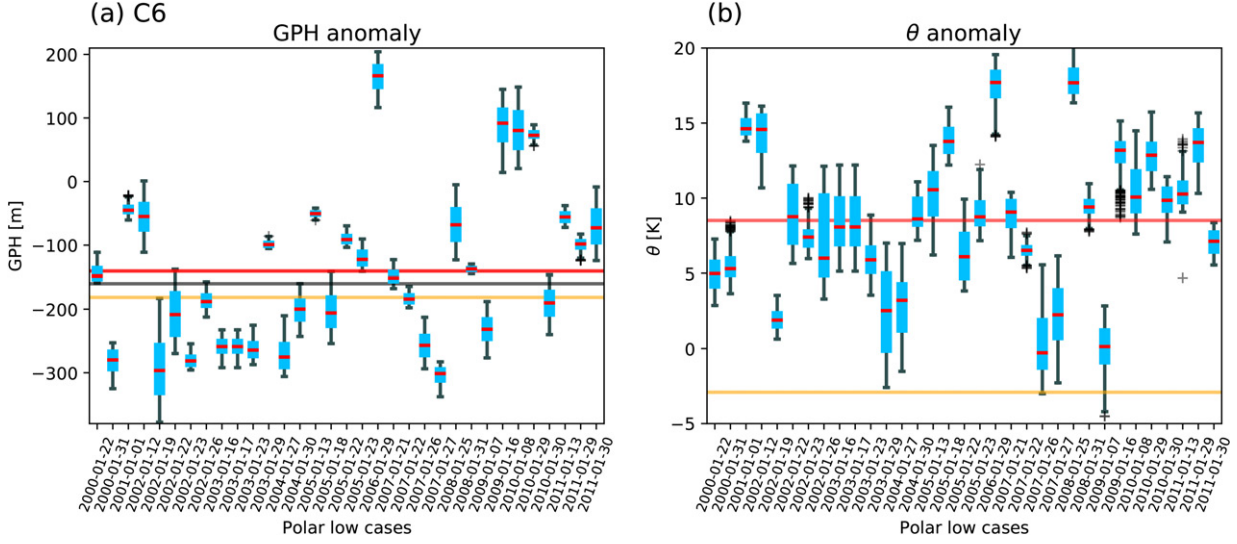
Fig. 8. Box plots for ASRv2 grid points within a 200 km radius around the genesis point for each of the January cases between 2000 and 2011. Anomaly of the GPH at the 500 hPa level (a) and potential temperature at the 850 hPa level (b). Lines correspond to those in Fig. 3. Blue boxes indicate interquartile range (IQR) and black whiskers the 1.5IQR. Individual outliers are presented as the black crosses.
