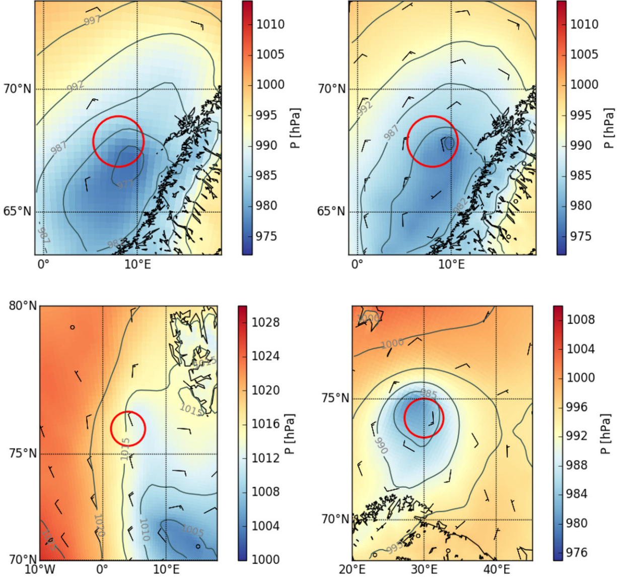
Fig. 2. MSLP (colour shading and grey counters every 5 hPa) and wind speed and direction (wind barbs) for PL cases on 29 January 2010 from ASRv1 (upper left) and ASRv2 (upper right) and for 22 January 2007 (lower left) and 30 January 2011 (lower right). Both cases in the bottom row were plotted using the ASRv2 data. The red circle indicates a 200 km radius around the location from NL list.
