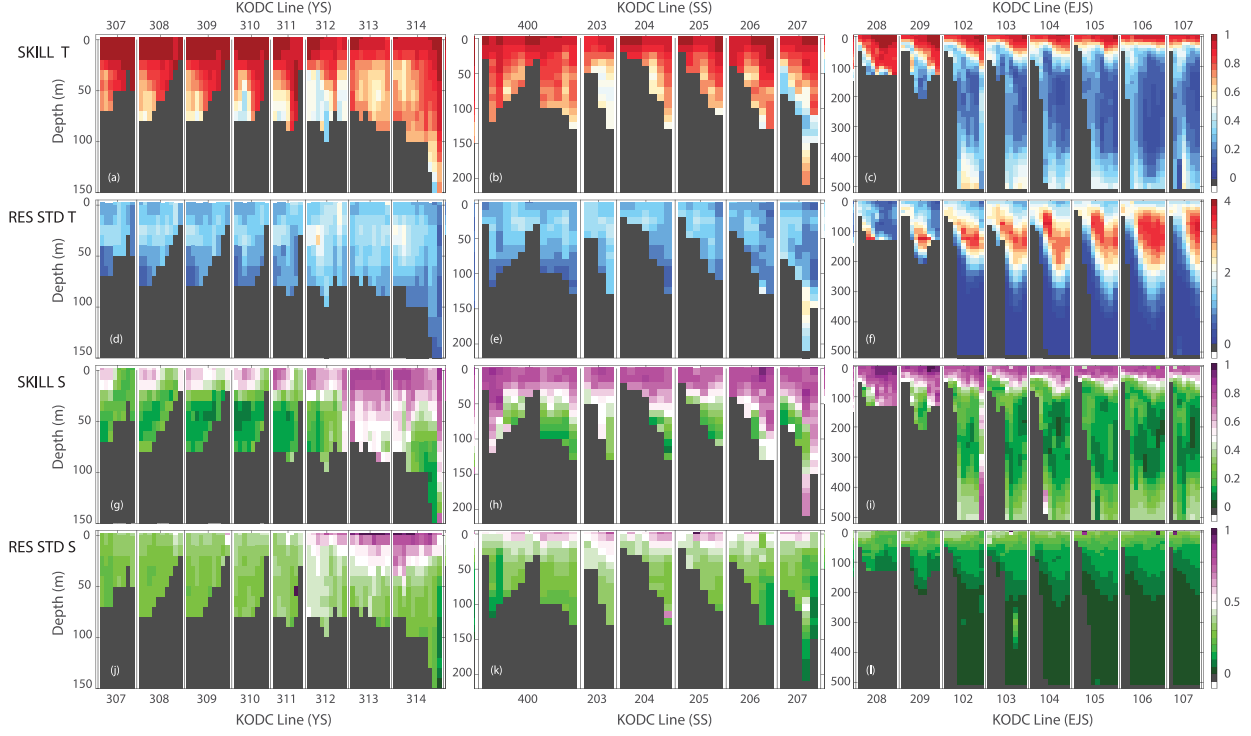
Fig. D1. Zonal sections of the total skill ( \kappa ) and standard deviation ( \langle d_R^2(t) \rangle^{1/2} ) of the residual temperature ( ^{\circ}\text{C} ) and salinity profiles sampled in the YS, SS, and EJS for a period of recent 20 years (1995 to 2014). (a–c) Total skill ( \kappa ) of the temperature. (d–f) Standard deviation ( \langle d_R^2(t) \rangle^{1/2} ) of the residual temperature. (g–i) Total skill ( \kappa ) of the salinity. (j–l) Standard deviation ( \langle d_R^2(t) \rangle^{1/2} ) of the residual salinity. (a), (d), (g), and (j): YS. (b), (e), (h), and (k): SS. (c), (f), (i), and (l): EJS. The vertical profiles are concatenated in terms of cross-shore lines, and the unsampled depths and bottom bathymetry are shown as gray columns.
