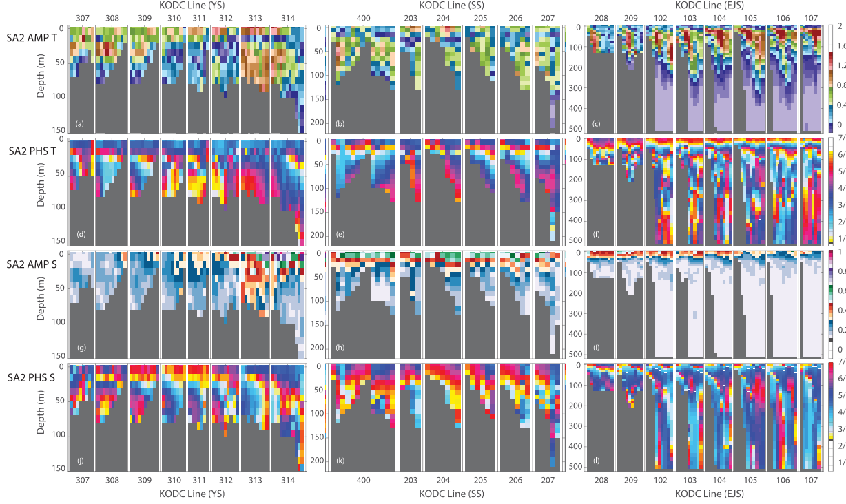
Fig. 5. Zonal sections of the semi-annual amplitudes and phases ( SA_2 ) of the temperature ( ^{\circ}\text{C} ) and salinity profiles sampled in the YS, SS, and EJS for a period of recent 20 years (1995 to 2014). (a–c) Semi-annual amplitudes of the temperature. (d–f) Semi-annual phases of the temperature. (g–i) Semi-annual amplitudes of the salinity. (j–l) Semi-annual phases of the salinity. (a), (d), (g), and (j): YS. (b), (e), (h), and (k): SS. (c), (f), (i), and (l): EJS. The vertical profiles are concatenated in terms of cross-shore lines, and the unsampled depths and bottom bathymetry are shown as gray columns. The phase is converted into the month of the year.
