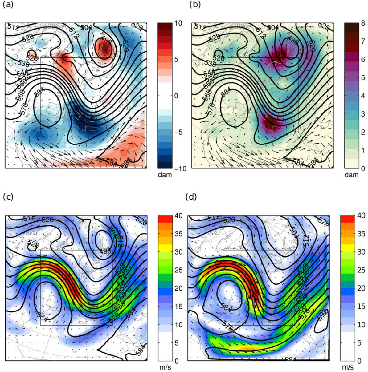
Fig. 5. (a) As Fig. 1c, but for model configuration LARGE. (b) As Fig. 1d, but for model configuration LARGE. (c) ECHAM fields as Fig. 1a, but for the domain of model configuration LARGE. (d) Variables as in Fig. 1a, but for the ensemble mean of the CCLM configuration LARGE. The area covered by the model configuration REF is indicated by rectangle in solid black lines.
