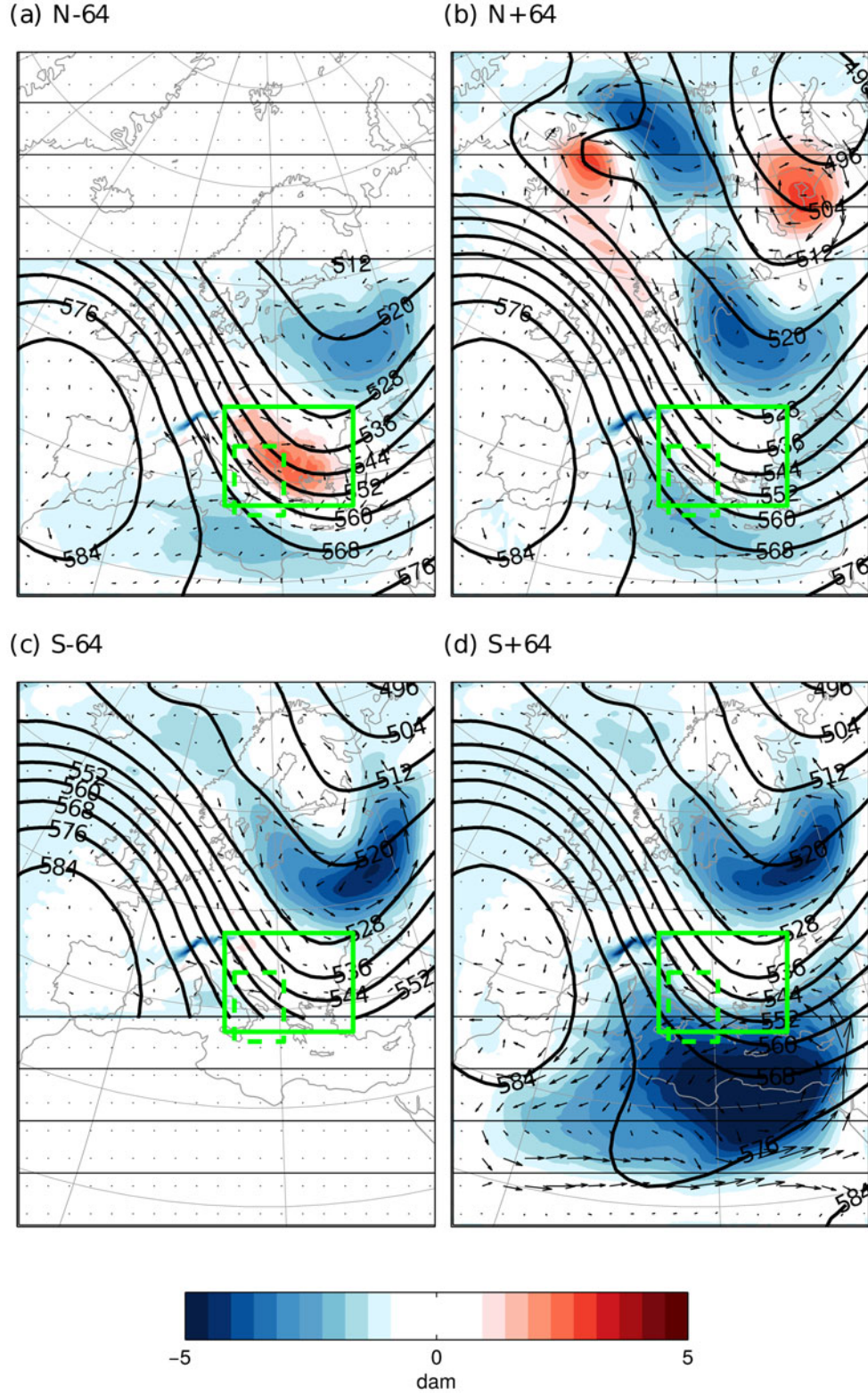
Fig. 3. As Fig. 1c, but for model configurations with shifted (a,b) northern and (c,d) southern model boundaries. Five horizontal solid black straight lines (including the outermost boundary) represent the five different locations of each lateral boundary with a distance of 32 grid boxes.
