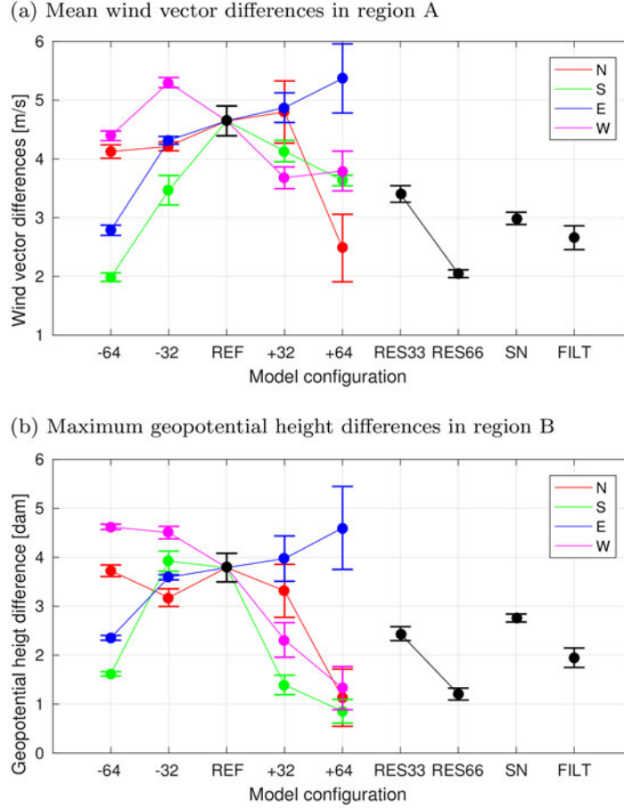
Fig. 4. (a) Area mean of region A of the ensemble mean (points) and standard deviation (error bars) of the norm of the of wind vector differences between CCLM and ECHAM and (b) area maximum of region B of the ensemble mean and standard deviation of the geopotential height differences between CCLM and ECHAM at 500 hPa for different model configurations.
