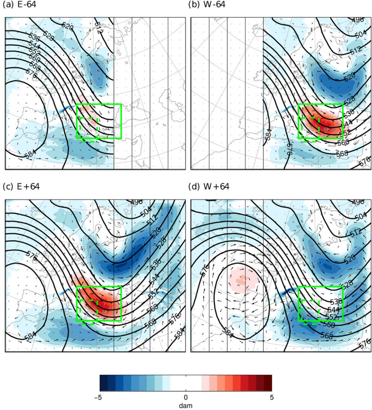
Fig. 2. As Fig. 1c, but for model configurations with shifted (a,c) eastern and (b,d) western model boundaries. Five vertical solid black straight lines (including the outermost boundary) represent the five different locations of each lateral boundary with a distance of 32 grid boxes.
