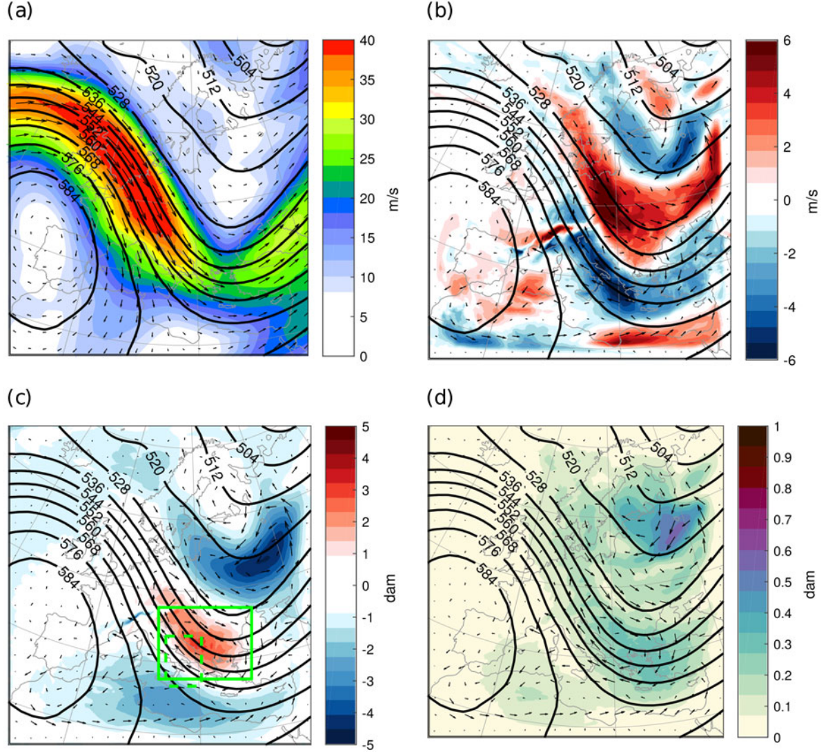
Fig. 1. Results of the reference configuration REF based on temporal averages of the analysis period at the 500 hPa level. (a) ECHAM geopotential height (contour lines), wind vectors (arrows) and wind speeds (colours). (b) ECHAM geopotential height (contour lines), ensemble mean wind vector differences (arrows) and wind speed differences (colours) between CCLM and ECHAM. (c) ECHAM geopotential height (contour lines), ensemble mean wind vector differences (arrows) and geopotential height differences (colours) between CCLM and ECHAM. Green rectangles indicate region A (dashed green line) and B (solid green line). (d) ECHAM geopotential height (contour lines), ensemble mean wind vector differences (arrows) and ensemble standard deviation of geopotential height differences between CCLM and ECHAM (colours). The longest vector in b–d is 7.8 m/s.
