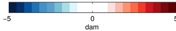
Fig. 6. As Fig. 1c, but for model configurations with different resolutions, spectral nudging and smoothed topography.
