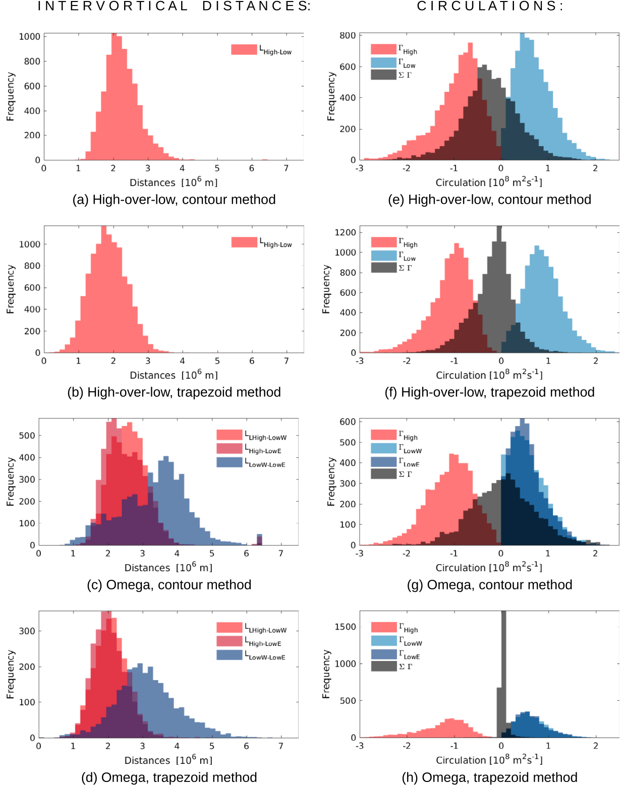
Fig. 5. Histogram of the distances l between the vortices (a-d) and the circulations \Gamma (e-h) of the single-time steps for High-over-low and Omega blocking as analysed with the (a,c,e,g) contour method and (b,d,f,h) trapezoid method. Due to overlapping distributions, the colours accordingly appear darker.
