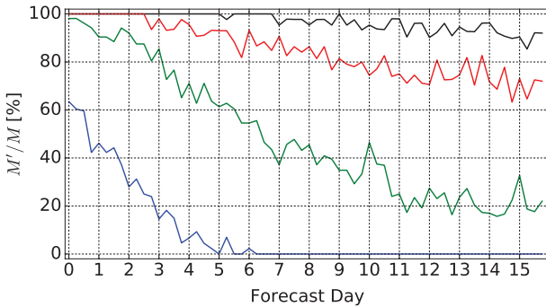
Fig. 5. Evolution of the percentage M'/M of the forecast cases for which K' \geq 2 for different values of a in the range from 0.6 to 0.9.
