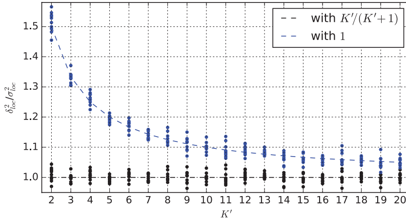
Fig. 2. Illustration of the effect of the normalization factor K'/(K' + 1) on the ratio of the estimates of the right- and left-hand sides of Equation (20). Notes: The values shown are based on randomly generated samples of 10,000 realizations of \mathbf{r}, \mathbf{r}_a, \mathbf{r}_f^k, k = 1, \dots, K' , assuming a Gaussian random distribution with mean \bar{\mathbf{r}} = \mathbf{0} . Because of the sampling fluctuations, the simulation is repeated 10 times for each value of K' and the results are shown by scatter-plots.
