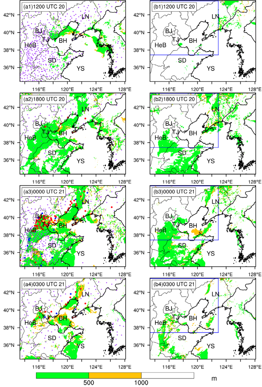
Fig. 2. Fog coverage (vis < 1000 m) from the simulation of the Truth Run (left) and BG Run (right, shading) at 12:00 UTC (a1, b1), 18:00 UTC (a2, b2) 20 February and 00:00 UTC (a3, b3) and 03:00 UTC 21 (a4, b4) February 2007, respectively, at the first model vertical level in the innermost model domain, and from the visibility observations by the surface stations (dots). The red, blue and purple dots denote observed visibility for the range of <500 m, 500–1000 m and > 1000 m, respectively. Abbreviations are the same as Fig. 1.
