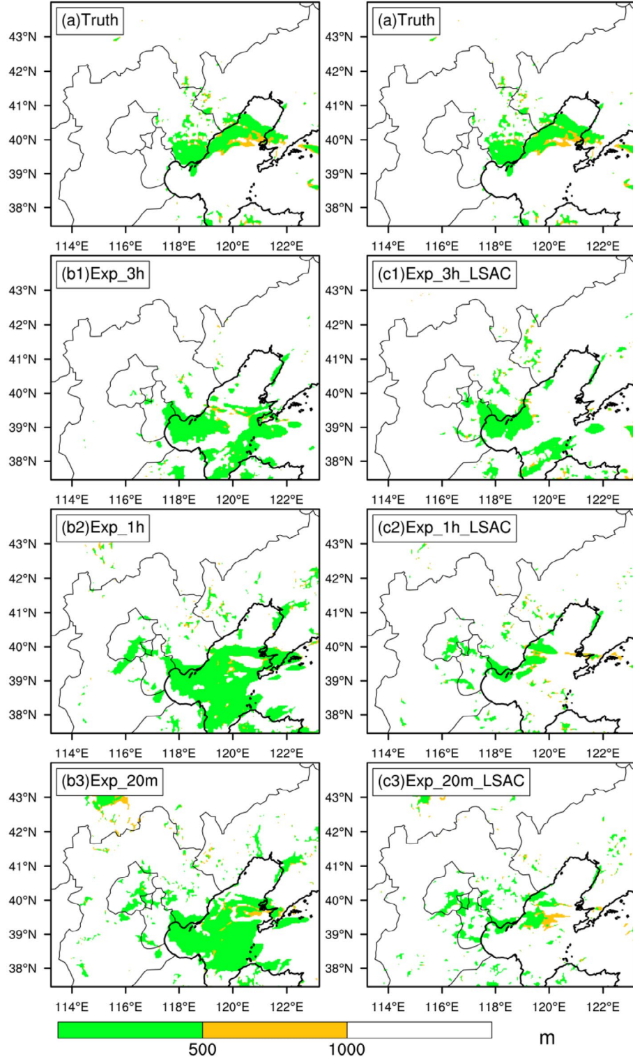
Fig. 6. As in the blue box of Fig. 2, but for the Truth Run (a) and the experiments Exp_3h (b1), Exp_1h (b2), Exp_20m (b3), Exp_3h_LSAC (c1), Exp_1h_LSAC (c2) and Exp_20m_LSAC (c3) in DNC at 12:00 UTC 20 February 2007 (1 h forecast).
