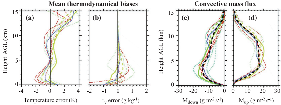
Fig. 11. Intercomparison of CRM simulations of 14-day mean profiles of temperature (a) and (b) water vapour mixing ratio biases relative to observations and convective downdraught (c) and updraught (d) defined in the same way in each run – each line corresponds to one model and the thick dashed lines in (c) and (d) are the average of CRM profiles – adapted from Xu et al. (2002), © Copyright 2002 RMS.
