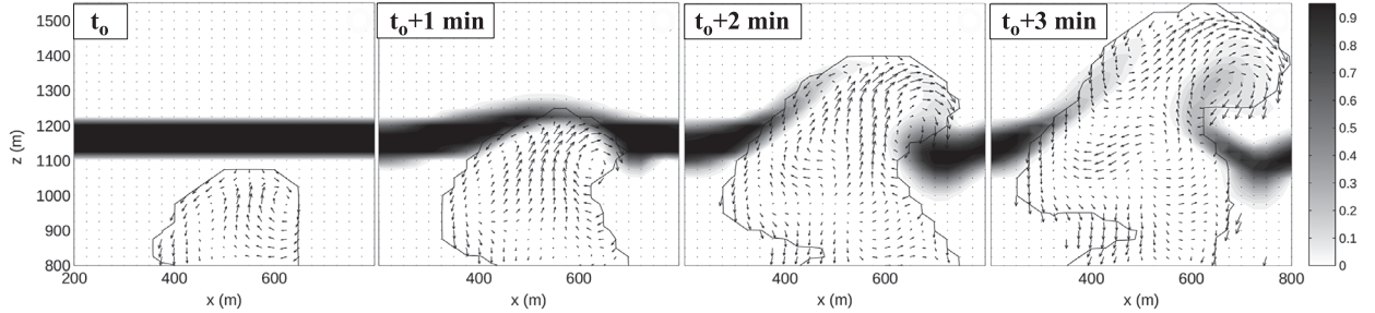
Fig. 13. Time sequence of four successive vertical cross-sections centred on the upper part of a growing cloud, with a 1-min frequency, starting t_o = 7.5 min after the initiation of the cloud. Arrows indicate wind in the cross-section. The contour delineates the cloud, defined as the area where the liquid water mixing ratio r_c is lower than 0.01 \text{ g kg}^{-1} . The shading indicates the mixing ratio of a tracer r_i introduced at the time of the first snapshot uniformly in a layer extending from 1100 to 1200 m at a 1 \text{ g kg}^{-1} concentration; Starting at t = t_o + 1 min (b), the cloudy air penetrates and deforms this layer, and transports the tracers upwards, mainly on the edges of the cloud – adapted from Zhao and Austin (2005), © Copyright 2005 AMS.
