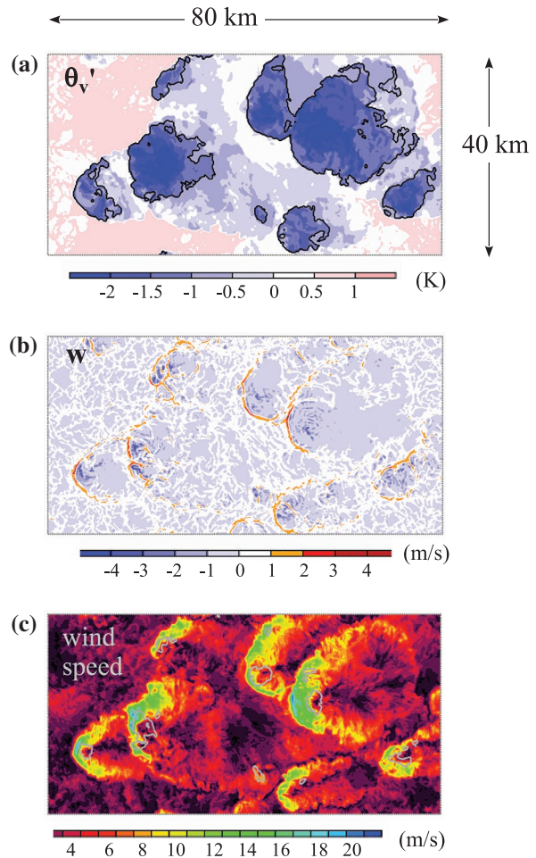
Fig. 14. Horizontal cross-section of potential temperature anomaly (a), vertical velocity (b) and wind speed (c) close to the surface, from a LES of deep convection over land. The figures illustrate the properties of the convectively generated cold pools: pools of negative temperature anomalies (a) with strong upward motion at their front – narrow orange stripes in (b) – and horizontal wind gusts – green and blue zones in (c).
