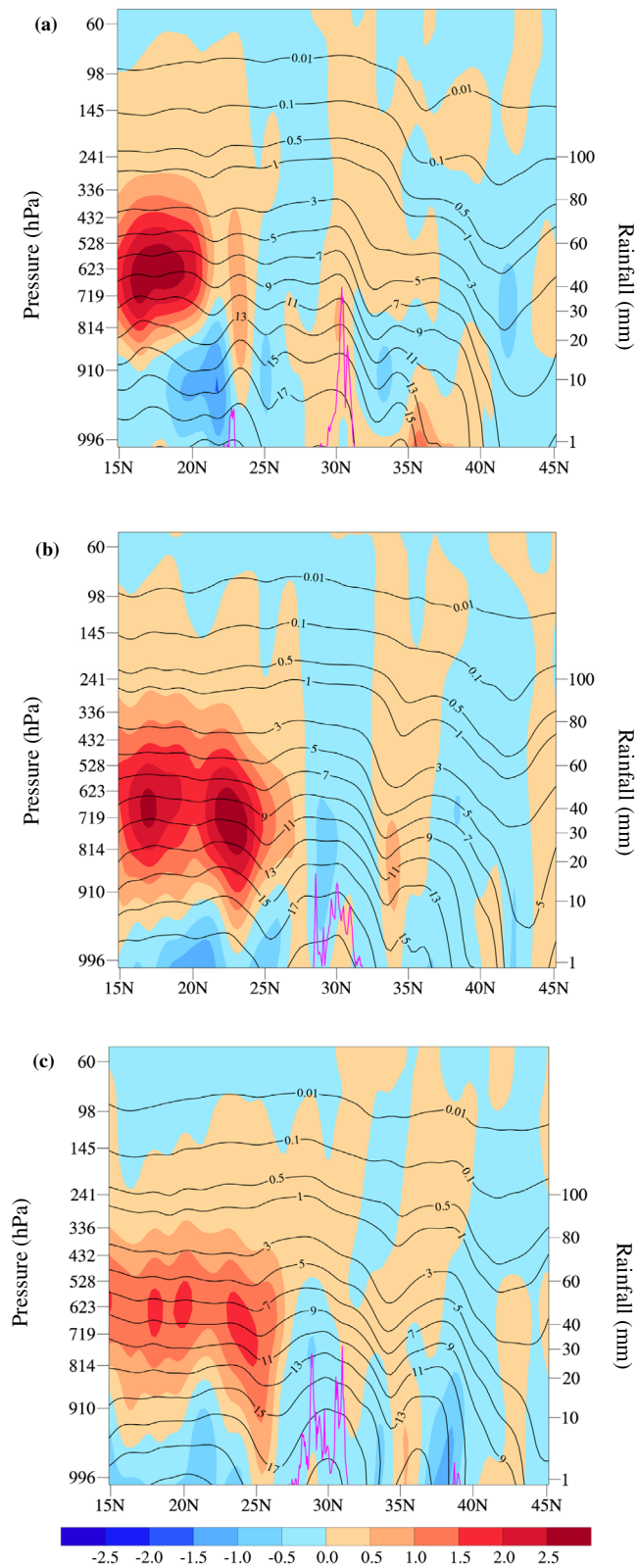
Fig. 10. Vertical and latitudinal cross sections along the 115E longitude for the analysis of water vapor mixing ratio of the AHIA experiment (contour interval: 1 \text{ g kg}^{-1} ) and the forecast differences of water vapor mixing ratio between the AHIA and CONV experiments (AHIA-CTRL, shaded) at (a) 0000 UTC, (b) 1200 UTC and 1800 UTC 2 July 2016. The 3-h accumulative rainfall observations (purple curve) ending at (a) 0000 UTC, (b) 1200 UTC and (c) 1800 UTC 2 July 2016 are indicated by the y-axis on the right by a logarithmic scale.
