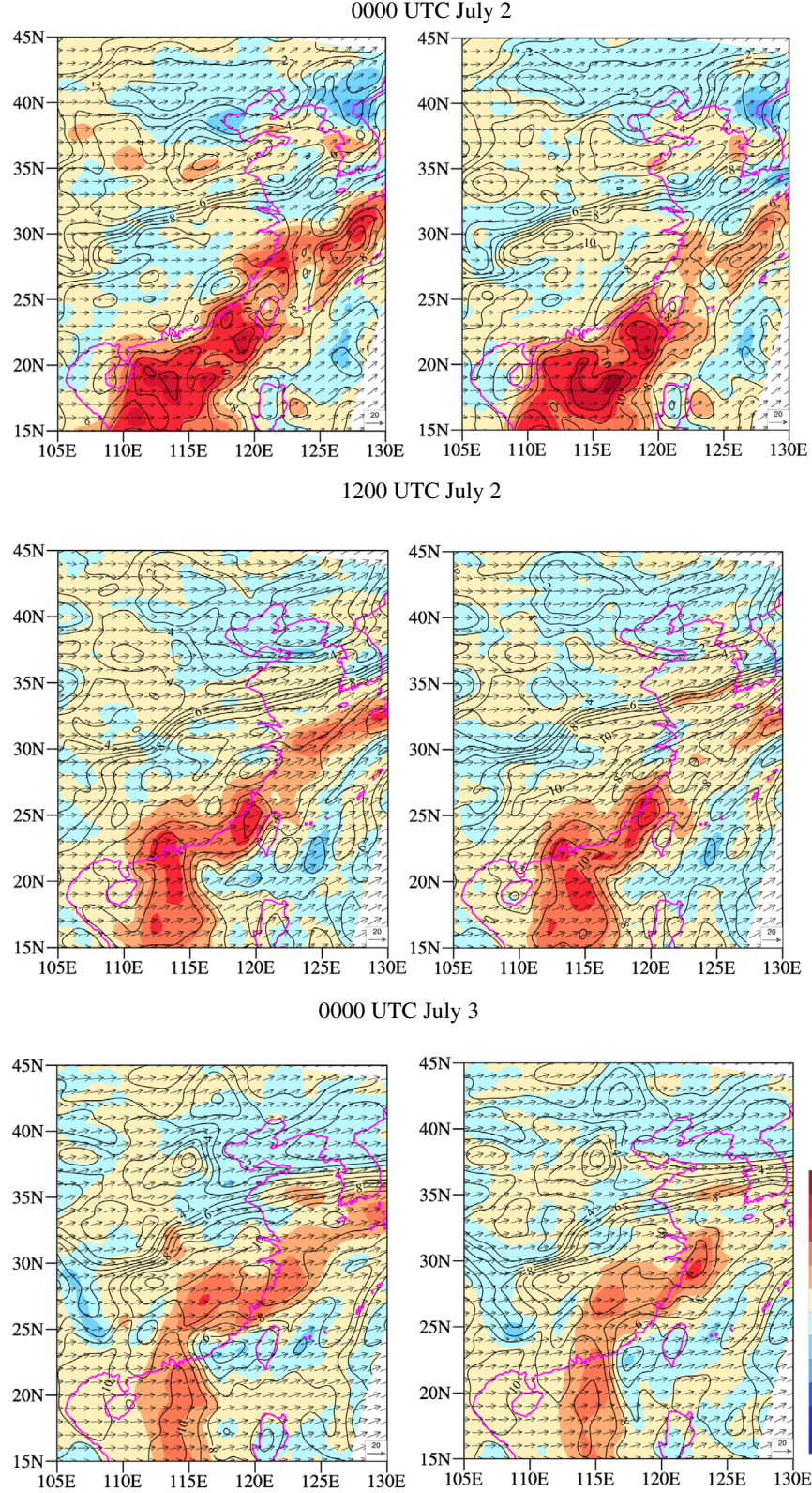
Fig. 9. Forecasts of water vapor mixing ratio at \sigma = 0.743 ( \sim 750 hPa) from the AHIA (left panels) and AHIG (right panels) experiments (contour interval: 1 \text{ g kg}^{-1} ), as well as the forecast differences between the AHIA and CTRL experiments (colour shading, left panels) and the forecast differences between the AHIG and CTRL experiments (colour shading, right panels) from 0000 UTC 2 July to 0000 UTC 2 July 2016 at 12-h interval.
