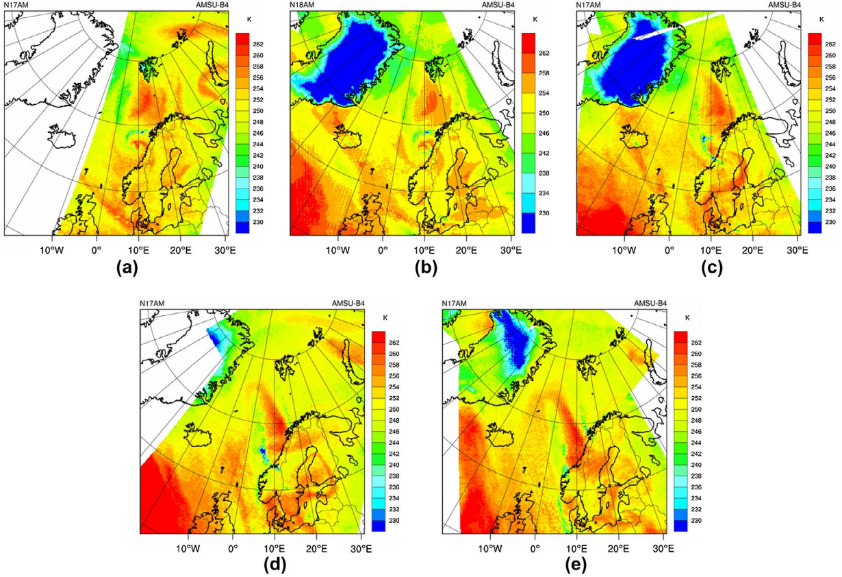
Fig. 7. AMSU-B channel 4 Brightness Temperature (in K) sequence for 20 November at around 09:00 UTC (a), 12:00 UTC (b), 18:00 UTC (c), and 21 November at 09:00 UTC (d), 18:00 UTC (e).
