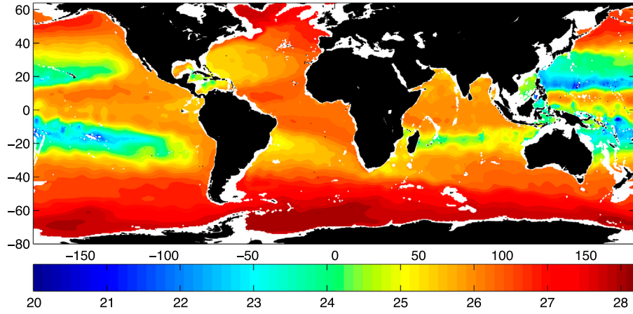
(c) abyssal neutral density ( \text{kg m}^{-3} )
