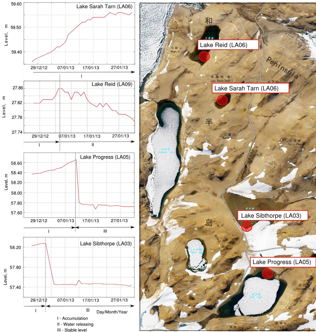
Fig. 10. The level changes on the lakes of different sizes at the Larsemann Hills. The image on the right is extracted from the orthomosaic with the scale 1:4000 (State Bureau, 2006).
