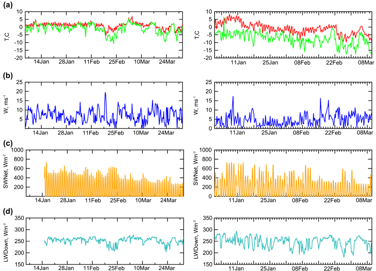
Fig. 4. Evolution of the meteorological forcing for the lake model FLake for the Fildes Peninsula (from station Bellingshausen) for the period the measurement campaign of 2012, right column, and for the Larsemann Hills (from station Progress) for the period the measurement campaign of 2014, left column: (a) screen level temperature (red line) and dew point (green line), °C; (b) wind speed W , m s -1 ; (c) calculated net shortwave radiation SWNet , W m -2 (the lake water albedo is constant and equal to 0.07); (d) calculated downward longwave radiation flux, LWDown , W m -2 . Here, all radiation fluxes are positive downward, from the atmosphere to the (lake water) surface.
