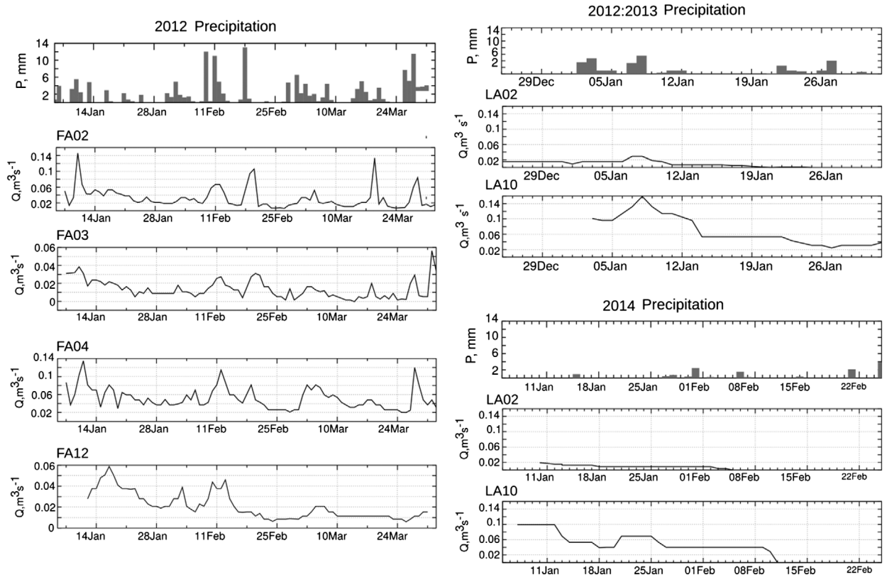
Fig. 9. The precipitation and water discharges measured by appropriate gauges at the rivulets on the Fildes Peninsula (left column) and the Larsemann Hills (right column).
