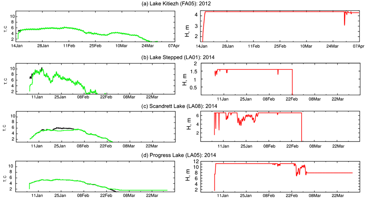
Fig. 6. The evolution during the periods of measurement campaigns of 2012 (the Fildes Peninsula) and 2014 (the Larsemann Hills) of the mean water temperature T_m (black line), bottom temperature T_b (green line) and mixed layer depth H (red line) as simulated by FLake for different lakes at these sites. See comments in the text.
