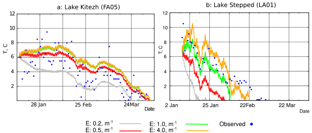
Fig. 3. Results of the sensitivity experiments of the modelled LWST to the light extinction coefficient ( E ). Lines of different colours show the evolution of the modelled LSWT with different values of E (according to the legend), blue dots show the observed LSWT for the period of the measurement campaign at the Fildes Peninsula for Lake Kitezh (FA05) (a) and at the Larsemann Hills for Lake Stepped (LA01) (b).
