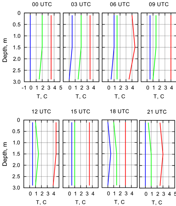
Fig. 7. The temperature profiles at different moments in time for Lake Stepped (LA01) for 2013: February, 5 (red line), February, 10 (green line), February, 23 (blue line).
