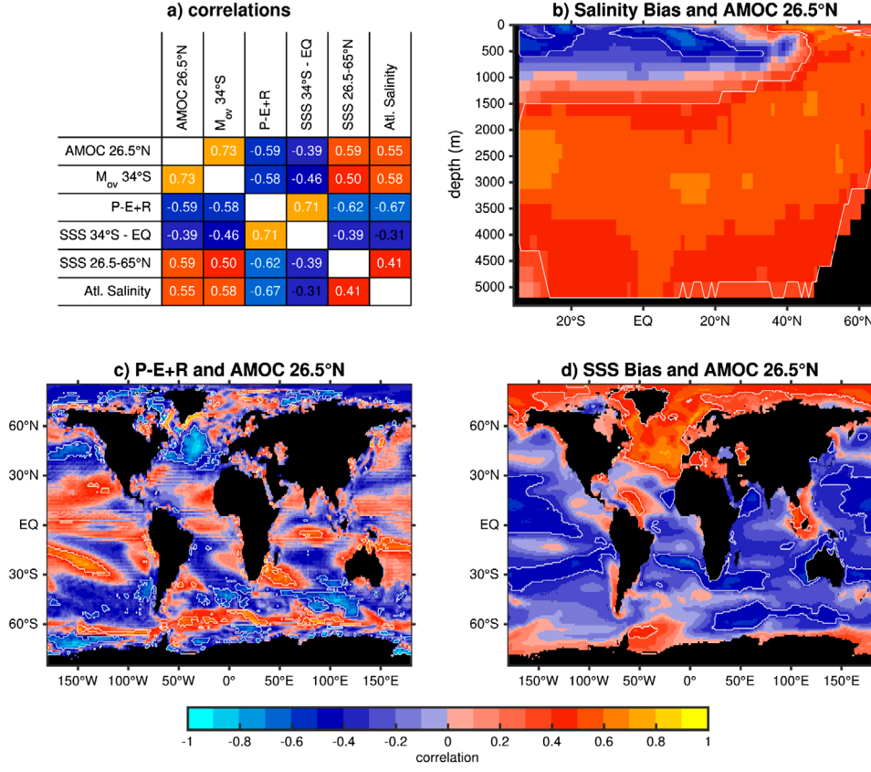
Fig. 7. (a) Correlations between AMOC at 26.5°N, M_{ov} at 34°S, integrated freshwater fluxes from Bering Strait to 34°S (P – E + R), South Atlantic SSS bias (SSS 34°S-EQ), North Atlantic SSS bias (SSS 26.5-65°N) and salinity bias in the full depth Atlantic from 34°S-65°N (Atl. Salinity). (b–d) Spatial patterns of correlations between AMOC at 26.5°N and (b) Atlantic zonal mean salinity bias, (c) P – E + R, and (d) SSS bias. Statistically significant correlations at the 99% level are circled in white (b,c,d) or written in white text (a). Only the CMIP5 models which have surface freshwater fluxes available were used to compute P – E + R (See Table 1).
