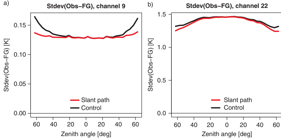
Figure 3. (a) Standard deviations of differences between observations and short-range forecast equivalents for channel 9 of ATMS as a function of the scan position (labelled here with the average satellite zenith angle). Black indicates the conventional treatment, red indicates statistics for calculations that take the slant-path geometry into account. The statistics cover the period 25 January to 24 February 2015, and are based on data over sea after cloud/rain screening. Biases have been removed based on bias corrections obtained from the underlying assimilation experiment that uses the conventional radiative transfer simulations. (b) As a), but for channel 22 of ATMS, the highest peaking humidity sounding channel.
