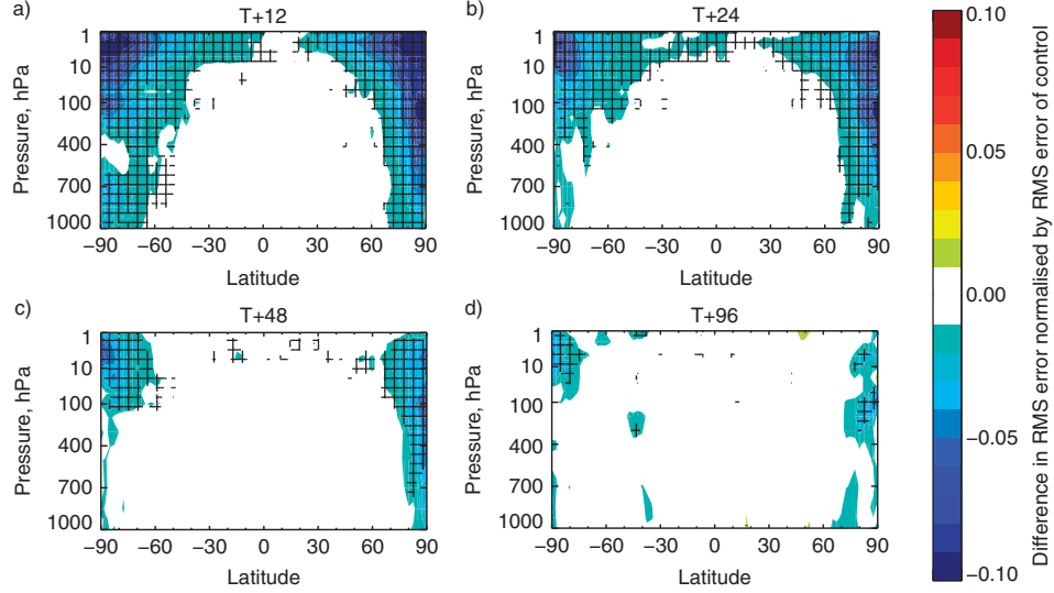
Figure 8. (a) Zonal means of normalised differences in the root mean squared vector wind analysis increments between the SlantPath experiment and the Control. Blue indicates a reduction in the standard deviation of the increments in the SlantPath experiment compared to the Control. Cross-hatching marks statistical significance at the 95% confidence level. (b) As (a), but for the root mean squared vector error of the 24-hour forecast verified against its own analysis. (c) As (b), but for the 2-day forecast. (d) As (a), but for the 4-day forecast. All statistics cover approximately 8 months over the two seasons combined, with a total of 430 to 468 samples.
