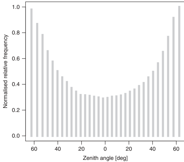
Figure 4. Normalised relative frequency of observations after geophysical quality control and after spatial thinning as a function of scan-position (labelled here by average zenith angle) for ATMS. The normalised relative frequency shown is the number of observations normalised by the maximum number of observations for any scan position.
