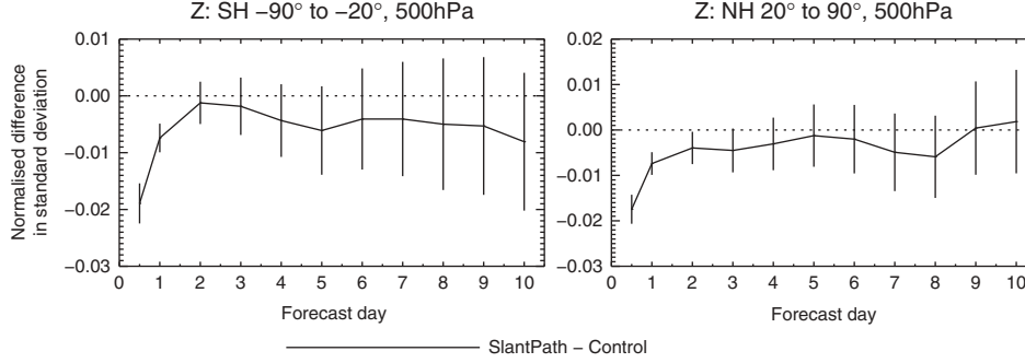
Figure 9. Normalised difference in the standard deviation of forecast errors in the 500 hPa geopotential as verified against each experiment's own analysis for the Southern Hemisphere extra-tropics (left) and the Northern Hemisphere extra-tropics (right). Vertical bars indicate 95% significance intervals.
