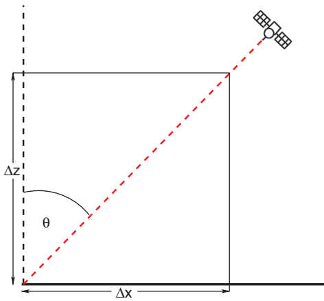
Figure 1. Schematic illustration of the satellite viewing geometry, viewing a location on Earth with a zenith angle of \theta along a slanted path through the atmosphere (red). The vertical profile currently used for radiative transfer calculations is indicated in black.
