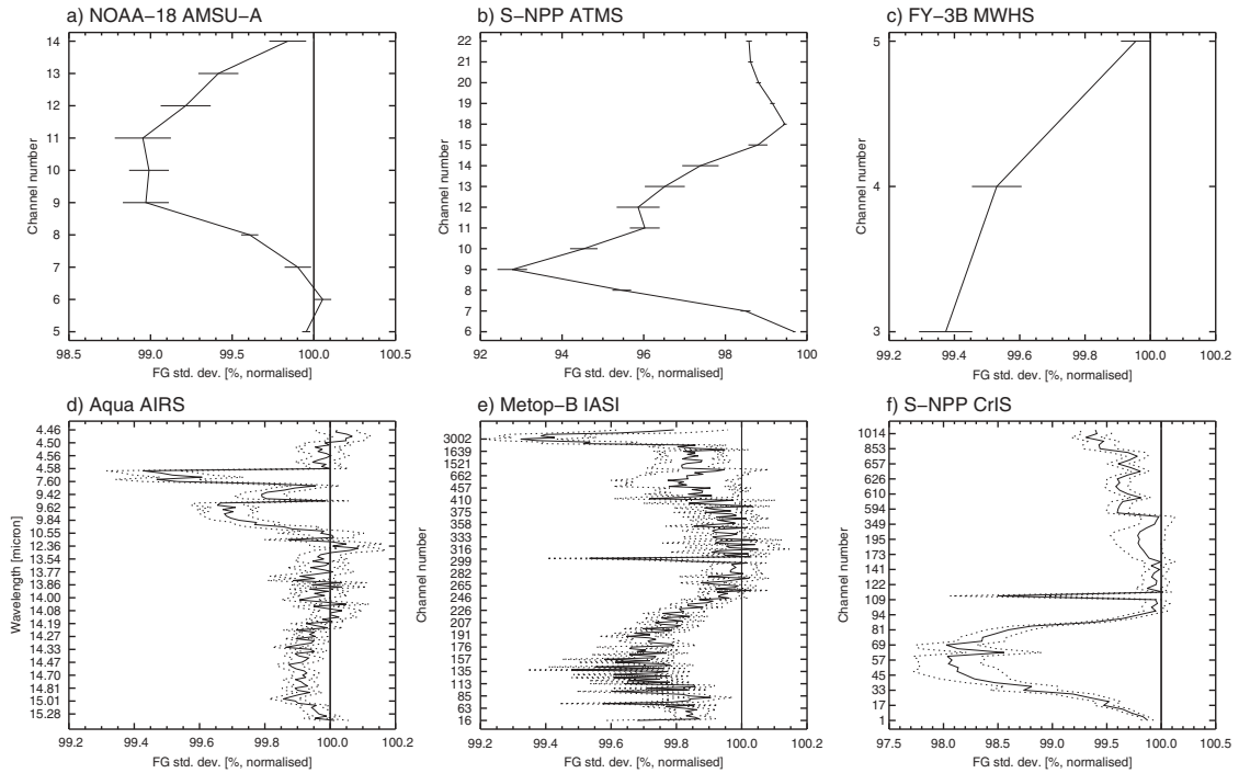
Figure 7. Standard deviation of differences between observations and simulations that take the slant-path geometry into account, normalised by equivalent values obtained with simulations that ignore the slant-path geometry. Values below 100% indicate smaller standard deviations when the slant-path geometry is taken into account. Horizontal bars indicate 95% significance intervals. Statistics are based on data covering the period 25 January to 24 February 2015, after quality control and thinning and after applying bias correction. The six panels show: (a) Statistics for AMSU-A on NOAA-18, (b) ATMS on S-NPP, (c) MWHS on FY-3B, (d) AIRS on Aqua, (e) IASI on Metop-B, and (f) CrIS on S-NPP.
