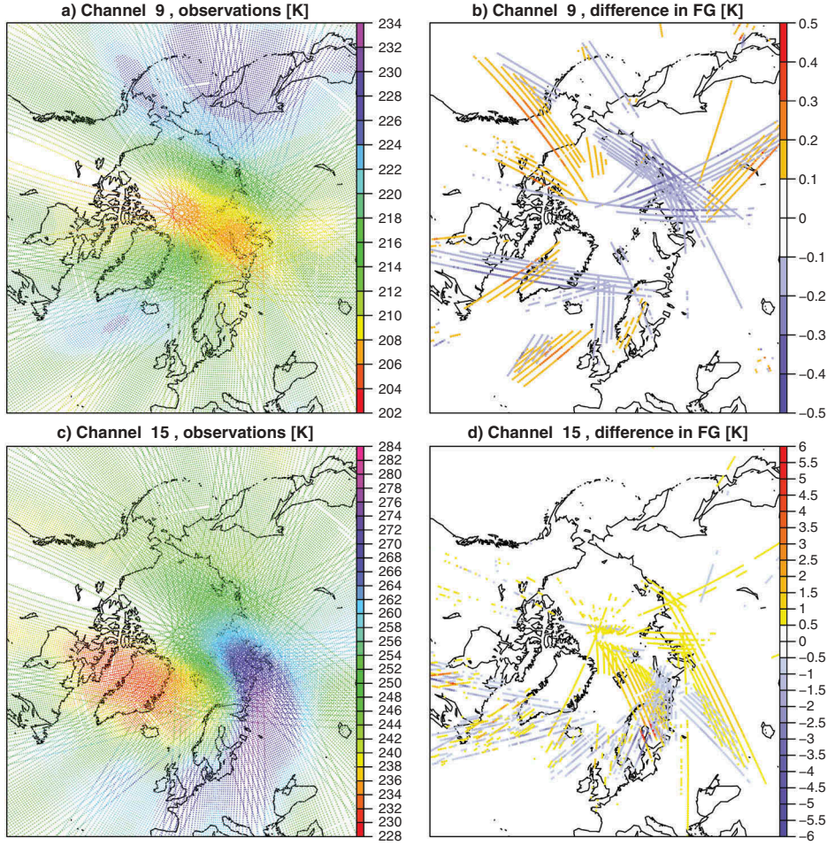
Figure 2. (a) Observed brightness temperatures [K] for ATMS channel 9 for a 12-hour period around 25 January 2015 00UTC. (b) Difference in the radiative transfer simulations from short range forecasts with and without taking the slant-path effect into account, for the observations shown in a). Note that only differences with an absolute value larger than 0.1 K are shown. (c) As a), but for channel 15 of ATMS. (d) As (b), but for the observations shown in (c). Note that only differences with an absolute value larger than 0.5 K are shown here.
