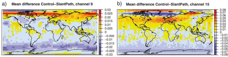
Figure 6. (a) Maps of the mean difference [K] between neglecting the slant-path geometry and taking it into account in the simulations from short-range forecasts for channel 9 of ATMS on S-NPP. Statistics are based on simulations from the same short-range forecasts, covering the period 25 January to 24 February 2015, after geophysical quality control applied to the underlying observations. (b) As (a), but for channel 22.
