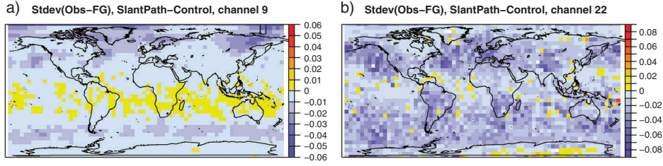
Figure 5. (a) Maps of the difference in the standard deviations of the departures [K] for channel 9 of ATMS between taking the slant-path geometry into account and neglecting the slant-path geometry. Negative values indicate a reduction in the standard deviations from taking the slant-path geometry into account. Statistics are based on simulations from the same short-range forecasts, covering the period 25 January to 24 February 2015, after geophysical quality control. Biases have been removed based on bias corrections obtained from the underlying assimilation experiment that uses the conventional radiative transfer simulations. (b) As (a), but for channel 22.
