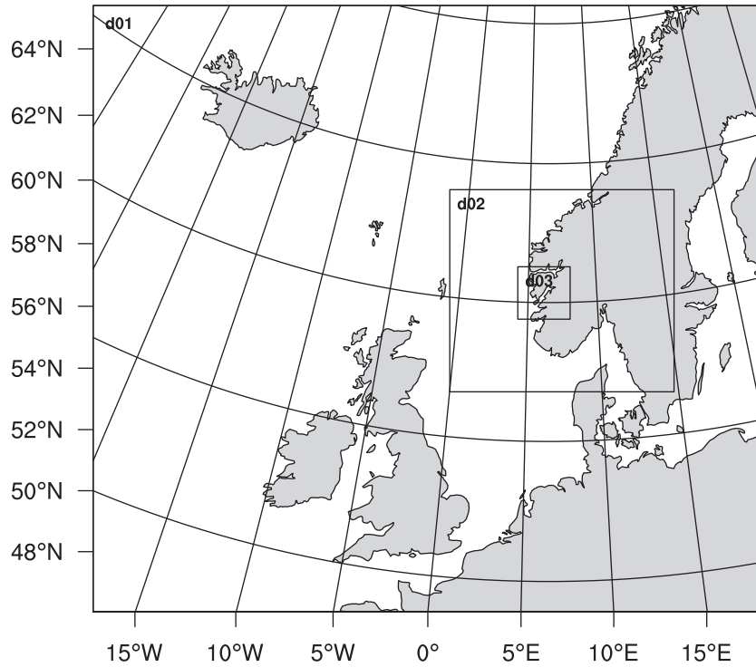
Fig. 2. Model domain set up for the WRF simulations. The domains d01, d02 and d03 have horizontal grid resolutions of 9 km, 3 km and 1 km, respectively.
