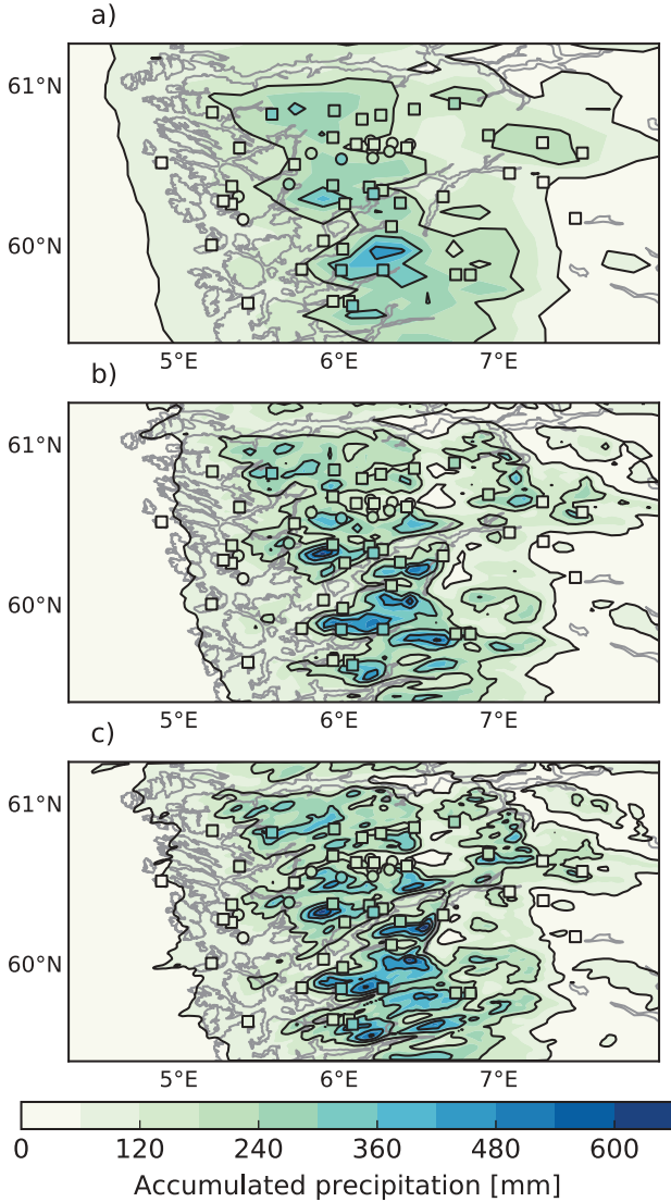
Fig. 10. Accumulated precipitation (25/06–29/06 October) in part of the 9 km grid (a). The circles correspond to the HOB0 stations, squares are stations from MET Norway. The inner parts of the markers show the observed accumulated precipitation amounts in the period. The other panels show the same for part of the 3 km domain in (b) and for the 1 km domain in (c).
