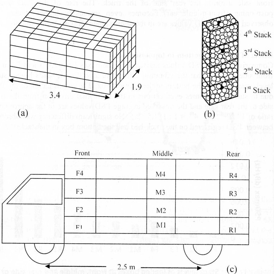
Figure 1. Pattern of stacking tomato boxes, (a) on the truck bed at the fully loaded configuration (b) in a single column (c) boxes selected from front, middle and rear stacks
