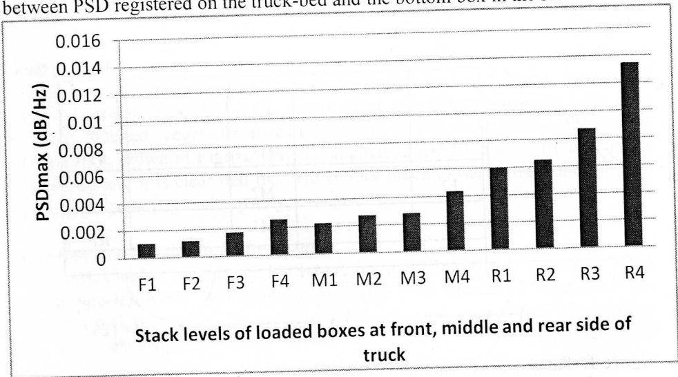
Figure 2. Summary of the results obtained on effective PSD levels of vertical vibration acceleration at different stack levels at front, middle, and rear of the truck bed. Average truck speed 20 \text{ kmh}^{-1} on fair road PSR 2 to 3 (or IRI 3.2 to 2 mm/m).
