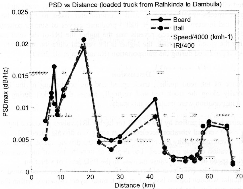
Figure 3. Vertical vibration acceleration (PSD) level as measured using, the accelerometer board (thick solid line), the instrumented sphere (thick dash line) during the transportation of truck from Rathkinda to Dambulla (distance 68 km). The variation of the speed of the truck (thin dash line; square edges) and the IRI of the road (thin dotted line; asterisk edges) are also marked using adapted scales.
