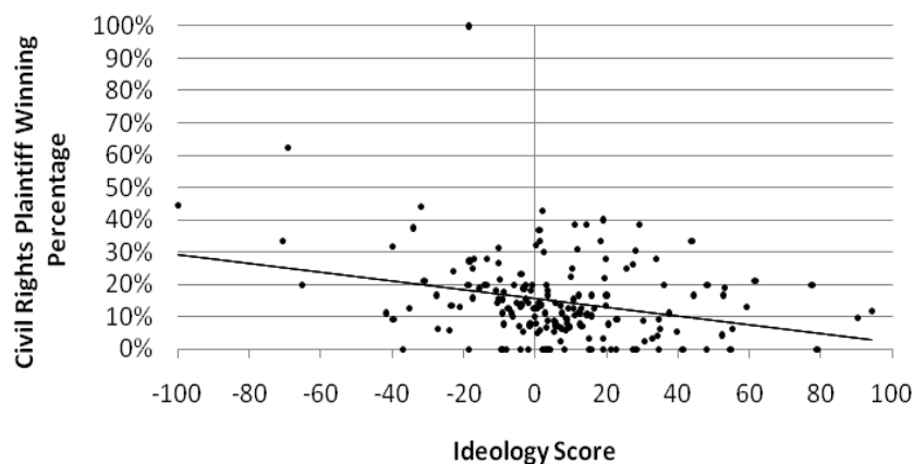
Figure 12 - Civil Rights Plaintiff Winning Percentage by Ideology Scores ( p=0.0007 )
