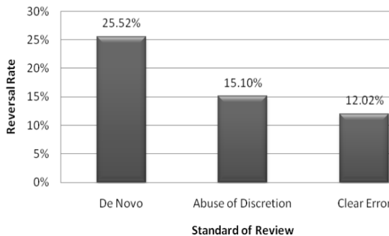
Figure 1 - Reversal Rate by Standard of Review (p=0.000)
