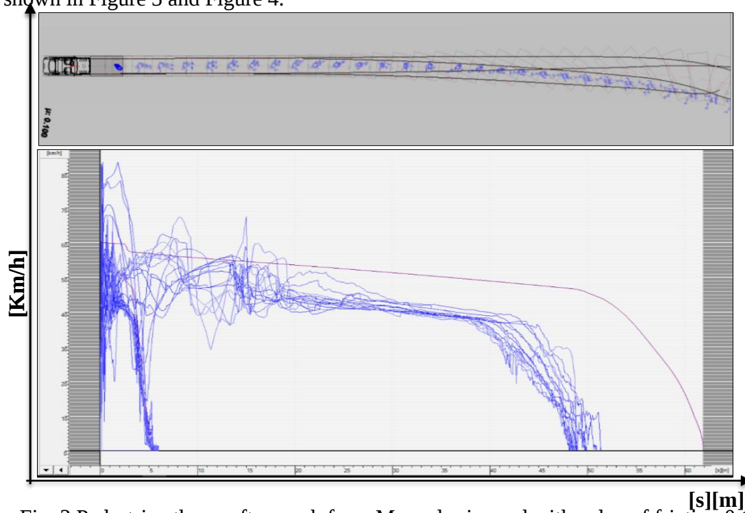
Fig. 3 Pedestrian throw after crash from Mercedes in road with value of friction 0.1
