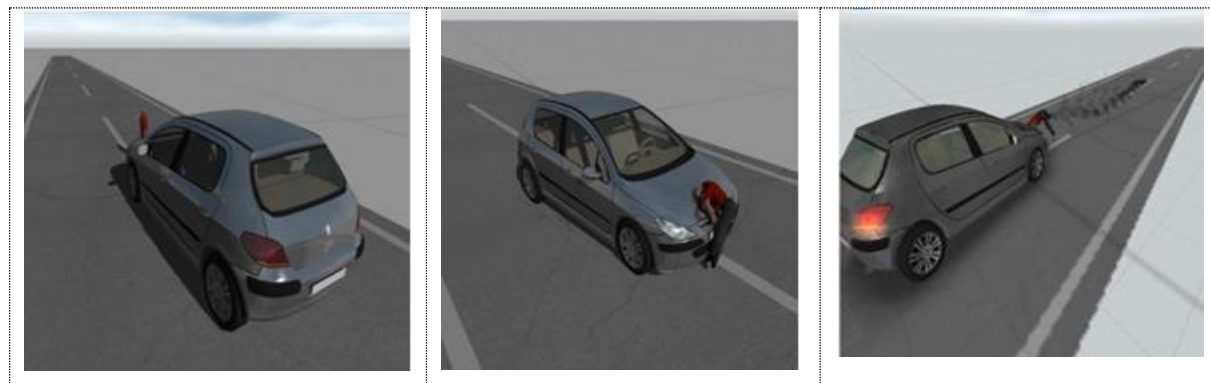
Fig. 5 Test-simulation of crash “Child- Peugeot 307”
