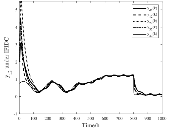
Fig. 7. Supply chain inventory y_{i2}(k) under IPIDC.
