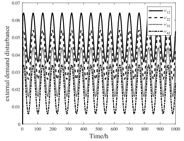
Fig. 3. External demand disturbance.
