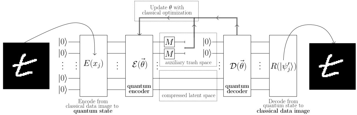
Fig. 3. Structure of a quantum autoencoder. Similarly to the classical version, there is an encoder part \mathcal{E} and a decoder part \mathcal{D} . We will also use the notation n - l - n to indicate that the input image is encoded using exactly n qubits, the latent space needs l qubits, and the output image is represented again by the n qubits.
