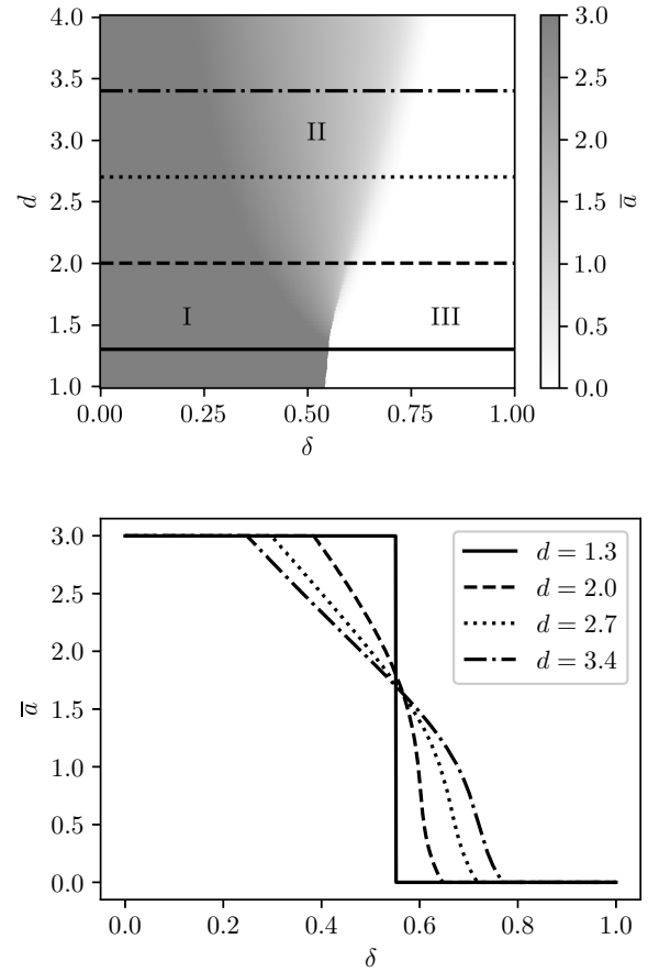
Fig. 6. Analysis for values of d \in [1, 4] , for constant \hat{\lambda} and \hat{f} as in Eqn. (22).
