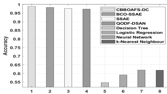
Fig. 12. Accuracy analysis of the CBBOAFS-DC model with existing techniques.
