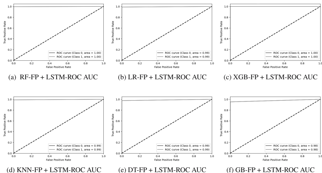
Fig. 3. ROC-AUC curves on the toddler screening dataset.
