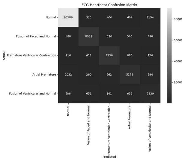
Fig. 7. Confusion matrix for ECG classification.
