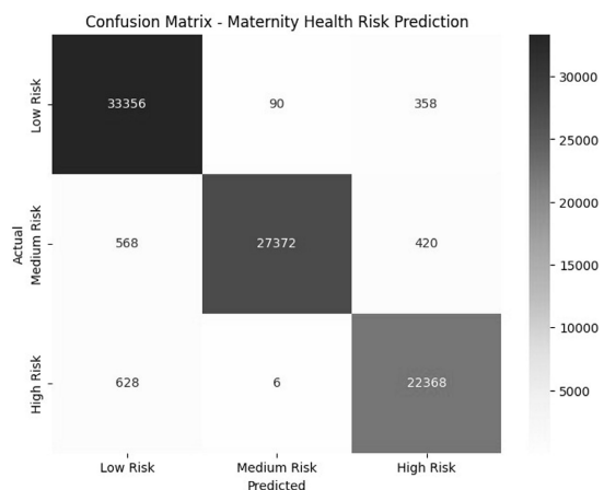
Fig. 3. Confusion matrix for maternity health textual data.
