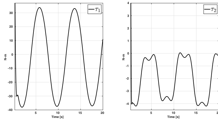
Fig. 6. Control responses \tau_1 and \tau_2 when tracking a smooth elliptic-shaped trajectory in the q_1 - q_2 -phase space; the inertia matrix M is partially known.
