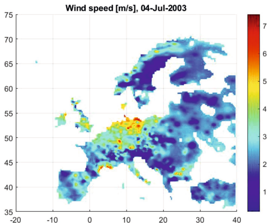
Fig. 2. Average daily wind speed for 2023-07-04 (own elaboration)
