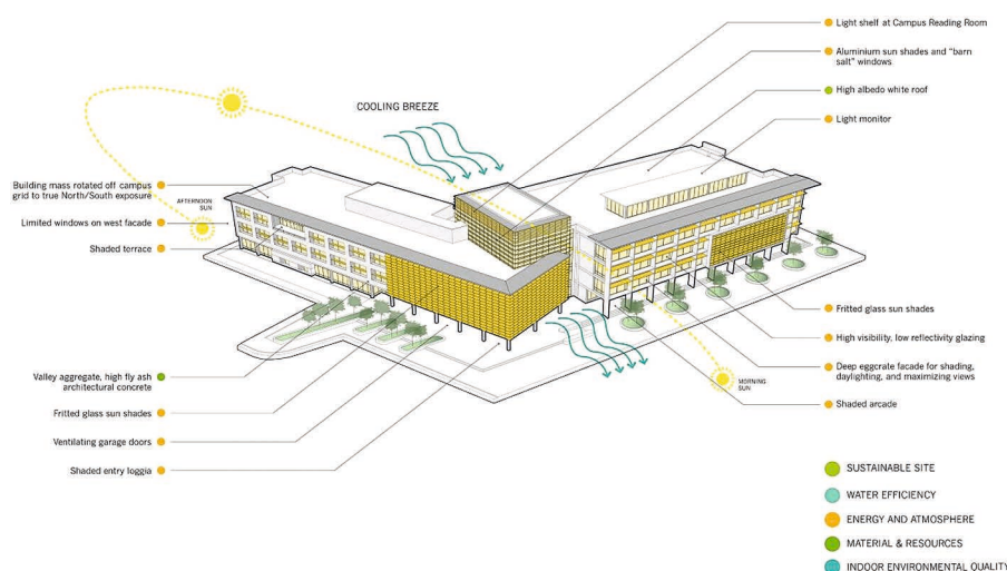
Fig. 2. The Leo and Dottie Kolligian Library – sustainability diagram (source: https://aeworldmap.com/2009/08/29/university-of-california-merced-library-and-information-technology-center-merced-california/ )
