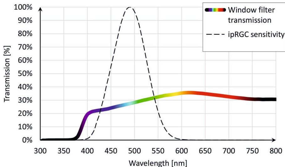
Fig. 4. Graph of spectral transmission of the example window with filter (source: own study)
