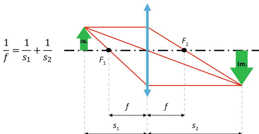
Fig. 12. Basic ray optics imaging principle (source: own study based on Landsberg 2003)
