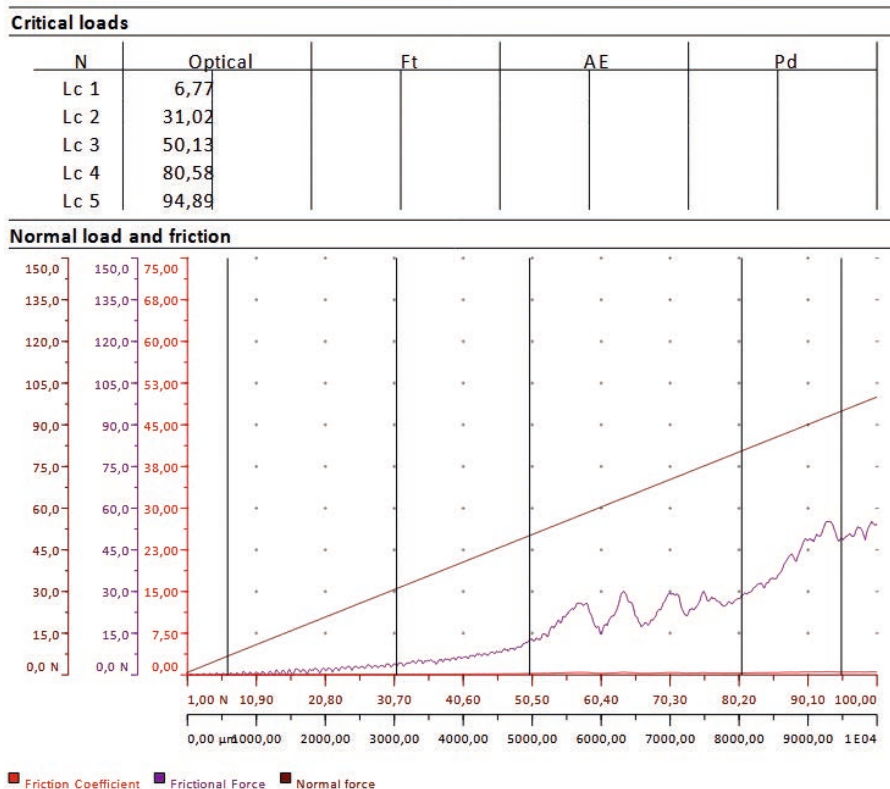
Fig. 3. Scratch test of DLC coated specimen (own elaboration)
