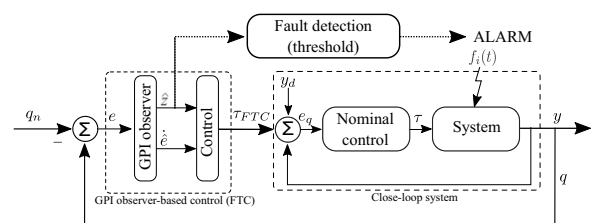
Fig. 5. Proposed FTC scheme.
