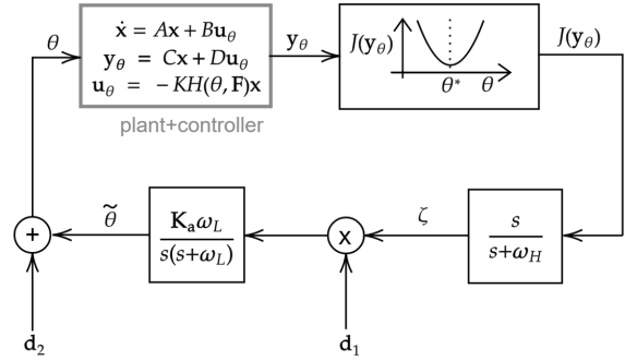
Fig. 8. Extremum seeking control framework.
