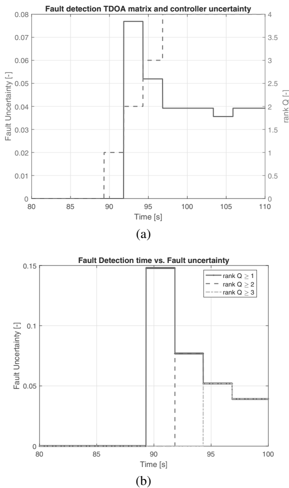
Fig. 13. FDD algorithm outputs: fault uncertainty (a) and uncertainty sensitivity (b) (a low magnitude incipient fault).
