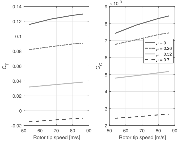
Fig. 4. Propeller thrust/torque coefficients for wind tunnel data.
