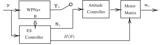
Fig. 9. ES controller within the ArduCopter software.
