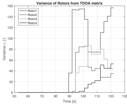
Fig. 12. Variance \alpha of the output of the \overline{Q} matrix during the execution of the FDD algorithm after the occurrence of a low magnitude incipient fault.
