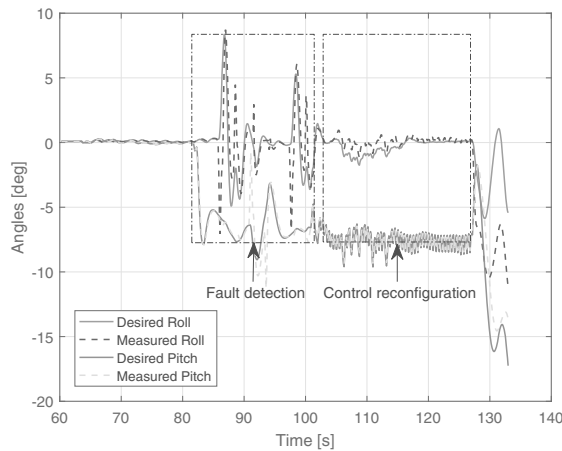
Fig. 16. Angles tracking during the fault-tolerant process.
