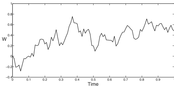
Fig. 4. Sample of Brownian motion.
