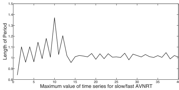
Fig. 8. Period length for a slow/fast AVNRT model.
