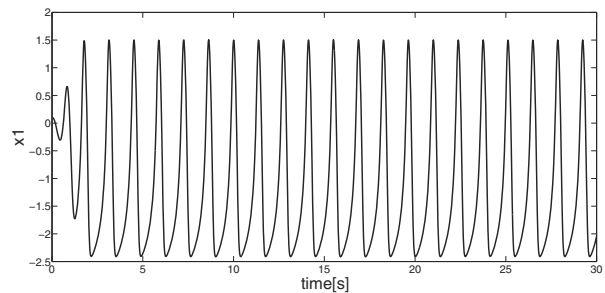
Fig. 5. Dynamics of action potential for the reference mvdP model, where the parameters are a = 5 , d = 3 , f = 3 , e = 7 .
